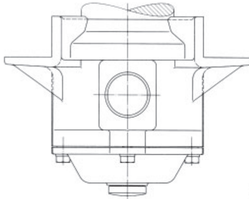
43: UIC axle boxes with cylindrical roller bearings
