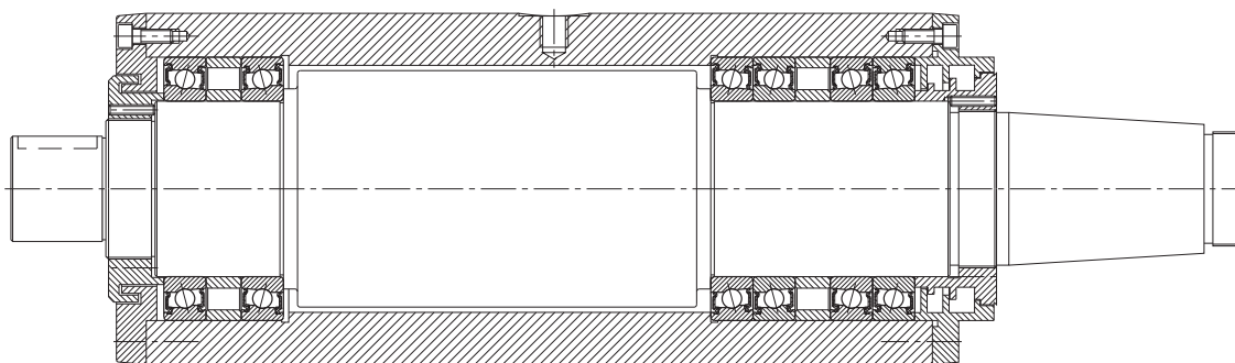
17: Bearing arrangement of an external cylindrical grinding spindle
