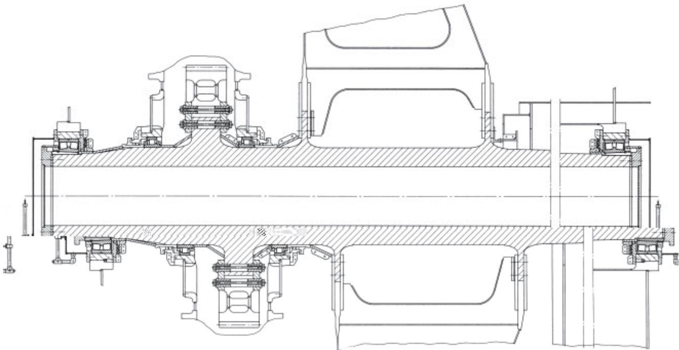
87: Bucket wheel mounting
