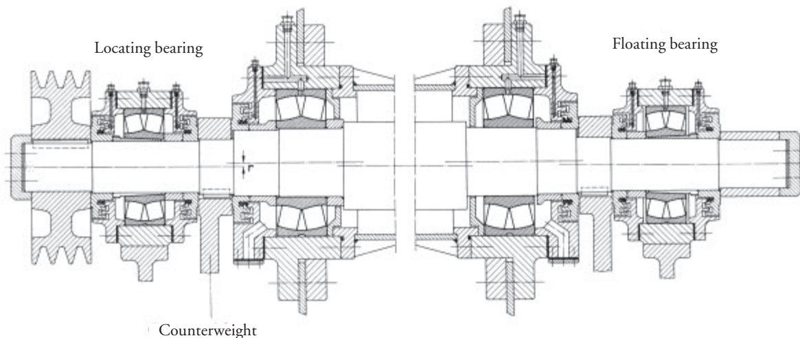
99: Four-bearing screen
