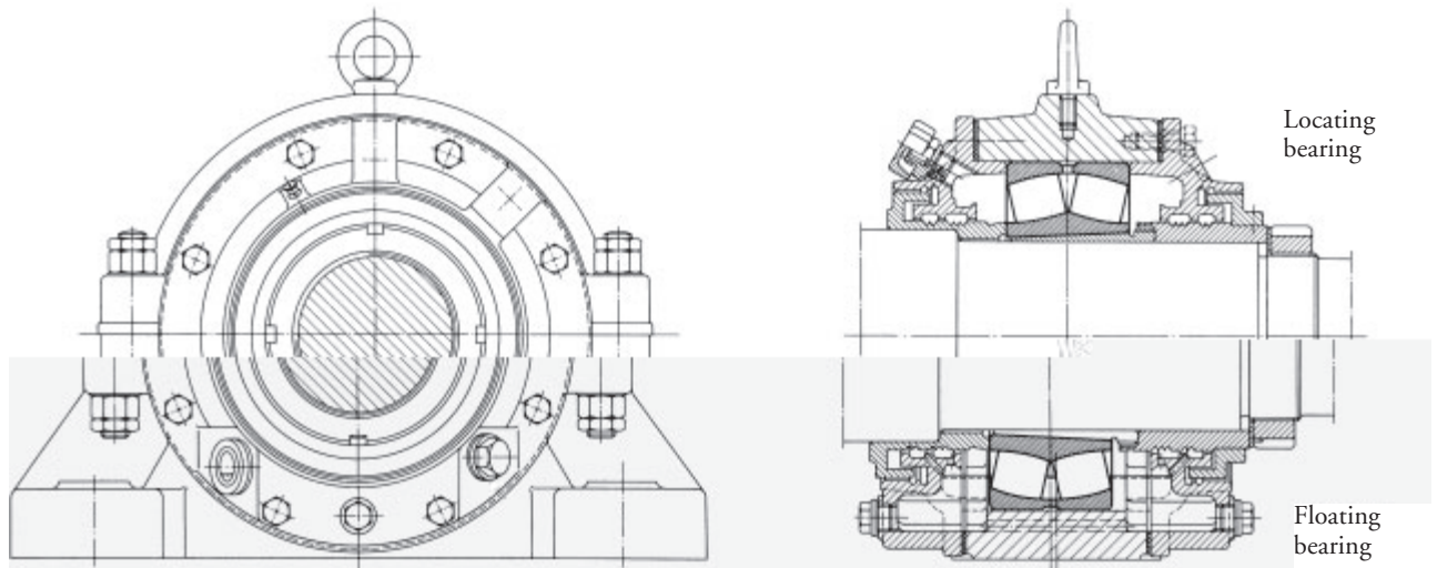
93: Hammer mill mounting
