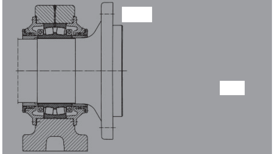
103: Locating bearing end with split spherical roller bearing
