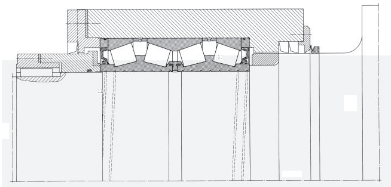
105: Work roll mounting for the finishing section of a four-high hot wide strip mill
