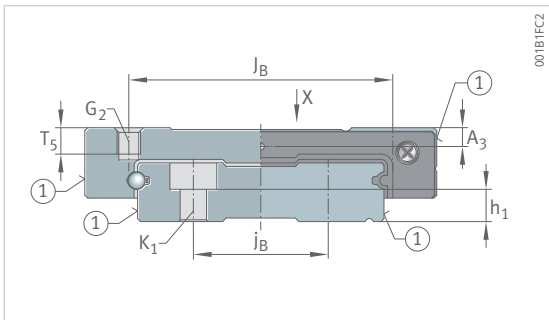
KUEM15-E-W
