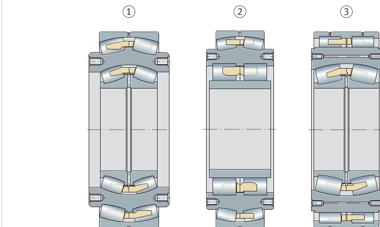
1 Triple ring bearings Z-5..04.DRGL for deflection-compensating rolls
