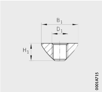
LEIS..T-NUT-SB-ST Swivel type
