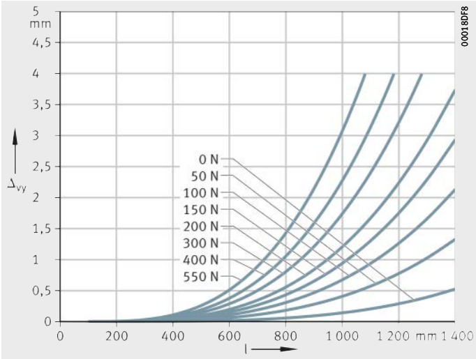
LTE16 Locating/locating bearing arrangement \Delta_{vy} = deflection l = support spacing Figure 10 Deflection about the z axis
