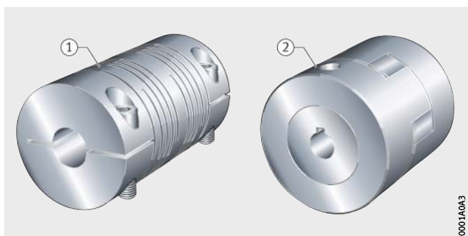
Figure 9 Couplings
