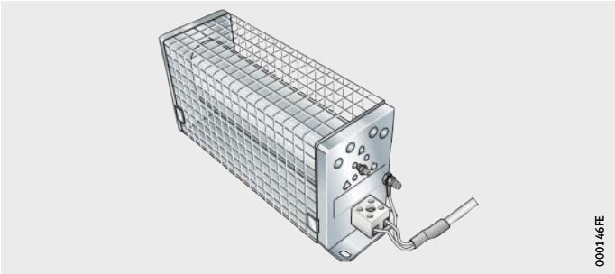
Figure 17 Ballast resistor
