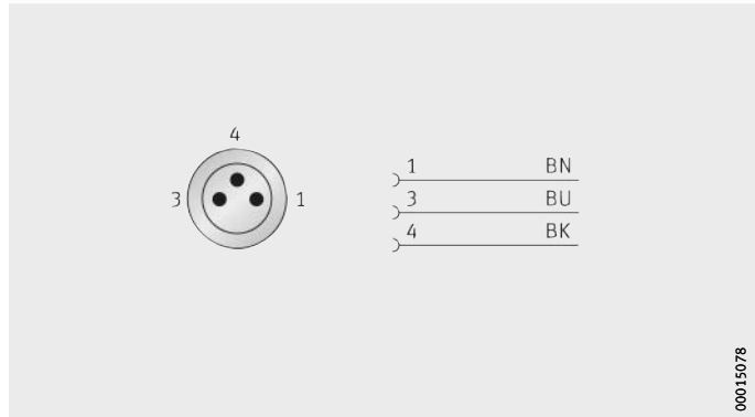
Figure 19 Assignment scheme
