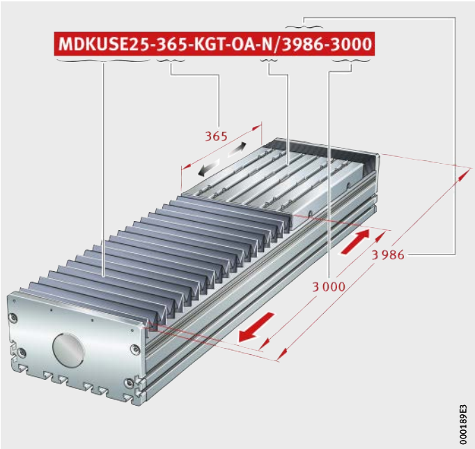
Figure 31 Ordering designation
