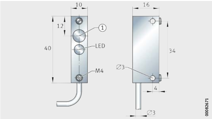
Figure 14 Dimensions of inductive limit switches
