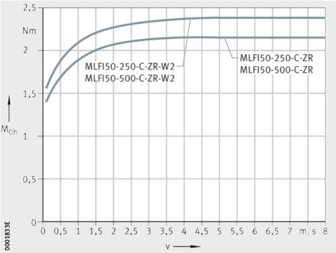
MLFI50.-C-ZR MLFI50.-C-ZR..W2 v = travel velocity of carriage M_{0h} = idling drive torque Figure 42 Idling drive torque Horizontal mounting position
