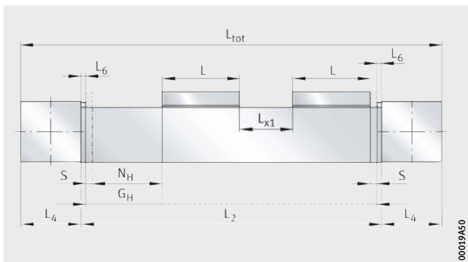
Figure 27 Length parameters for two carriages
