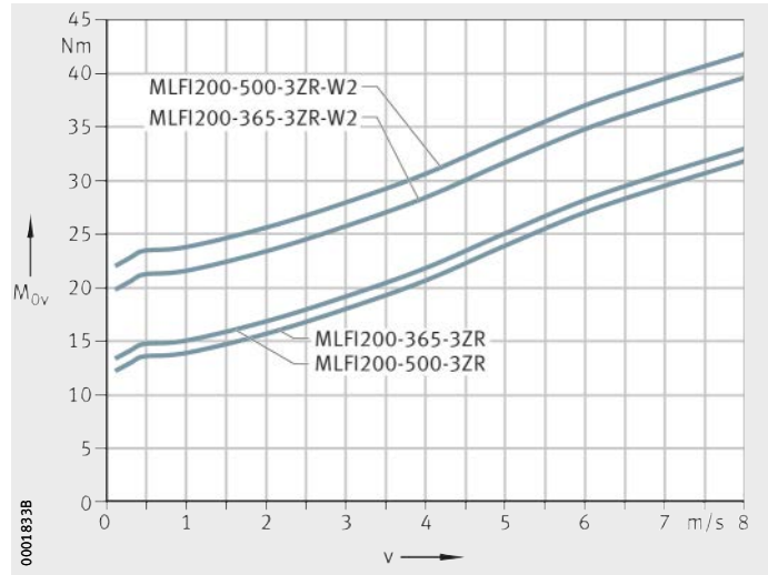
MLFI200...-3ZR MLFI200...-3ZR...W2 v = travel velocity of carriage M_{0v} = idling drive torque Figure 47 Idling drive torque Vertical mounting position
