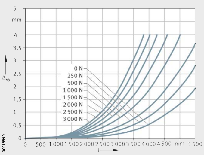
Figure 12 Deflection about the z axis
