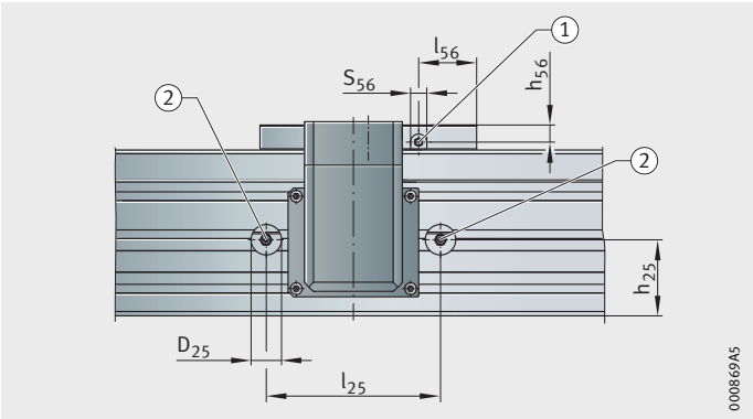
Figure 14 Lubrication points on long carriage unit
