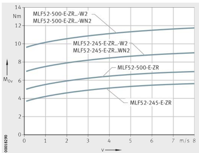
Figure 23 Idling drive torque Vertical mounting position
