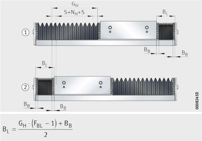
Figure 5 Effective length calculation
