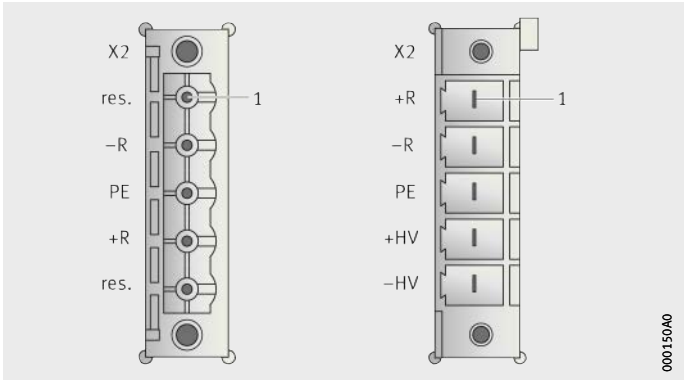
Figure 6 Plug X2
