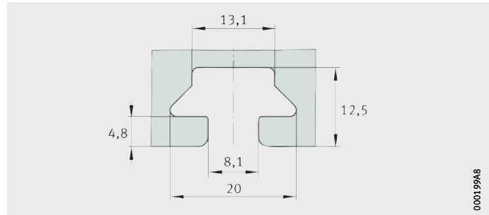
Figure 15 Dimensions of T-slots
