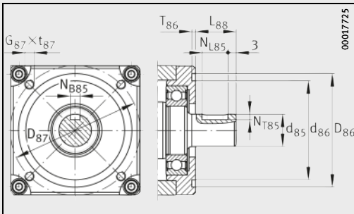
MLF..-ZR · Drive flange, drive shaft
