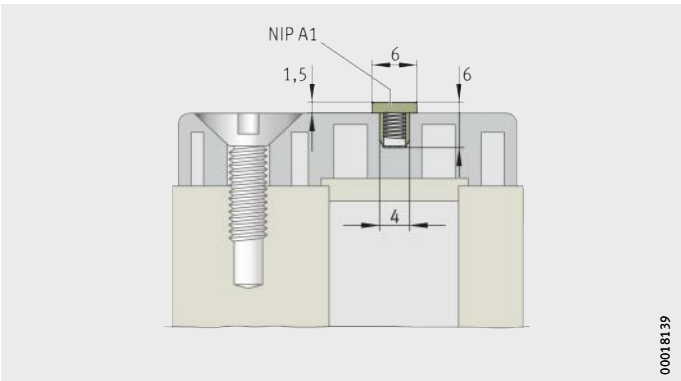
Figure 30 Mounting situation of the drive fit lubrication nipple NIP A1
