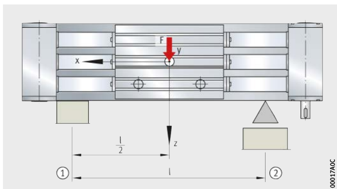
Figure 10 Deflection about the y axis
