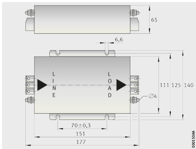
Figure 23 Dimensions
