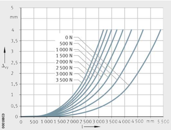
Figure 3 Deflection about the z axis
