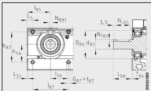
MKUVE15...-ZR · Drive flange, drive shaft
