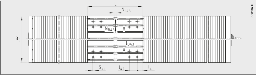
MDKUSE...KGT/...N, MDKUSE...KGT-OA...N · Top view, spacing between carriage units L \times 1 1)
