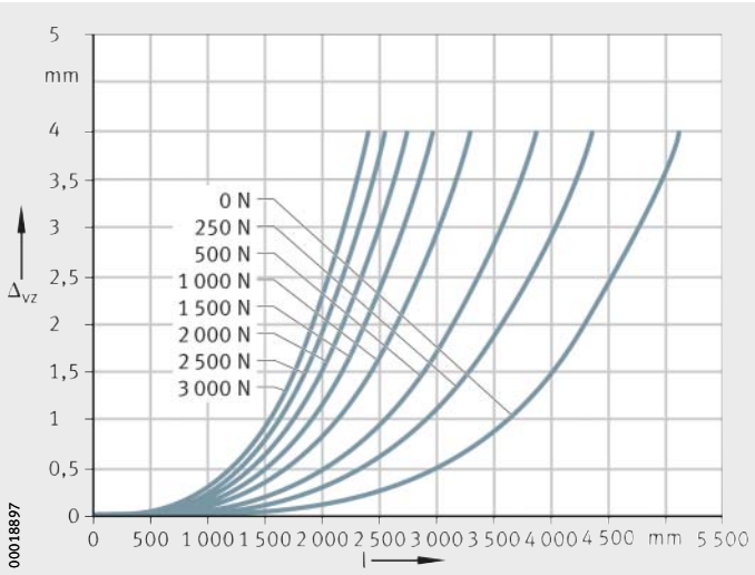
Figure 10 Deflection about the y axis
