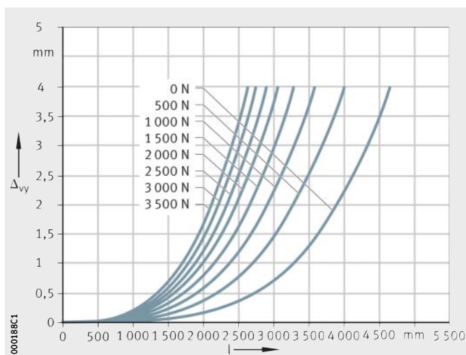
Figure 2 Deflection about the z axis
