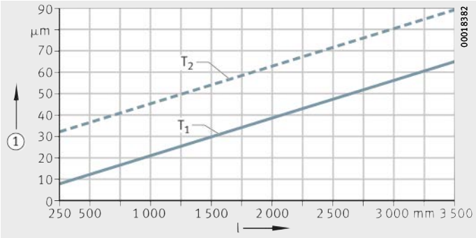
Figure 12 Accuracy values
