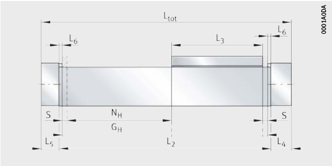
Figure 28 Length parameters for one carriage unit
