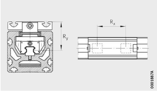
Mounting geometry of carriages
