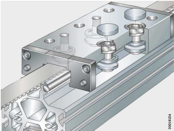
Figure 1 Carriage
