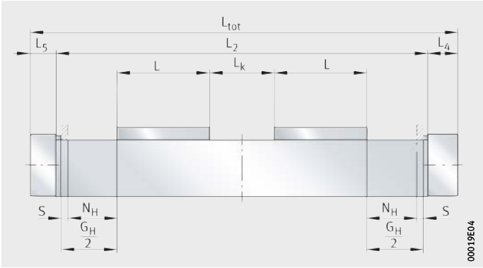
Figure 3 Length parameters
