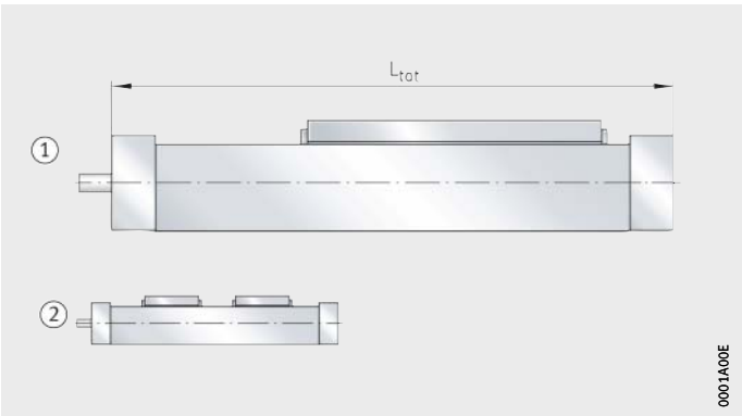
① Basic design ② Second carriage unit (WN2) Figure 33 Basic and additional designs
