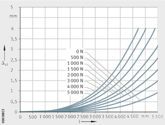
Figure 4 Deflection about the y axis
