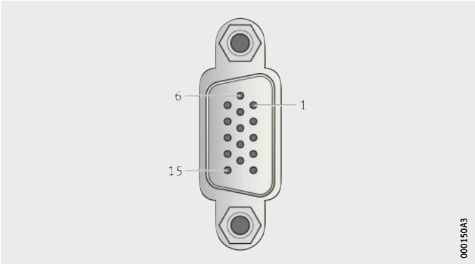
Figure 7 Plug X12
