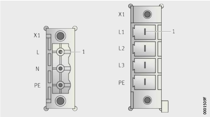
Figure 2 Plug X1
