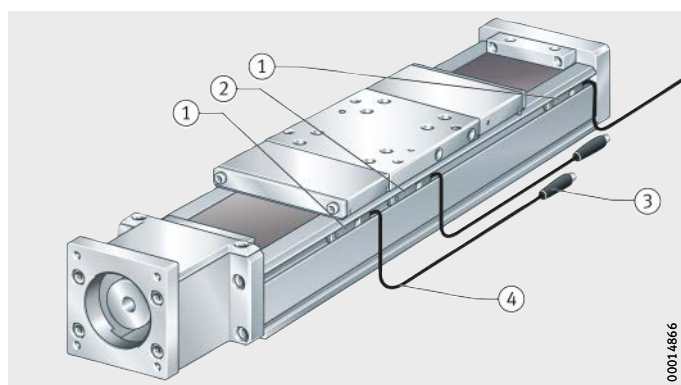
Figure 5 End position and zero point sensors
