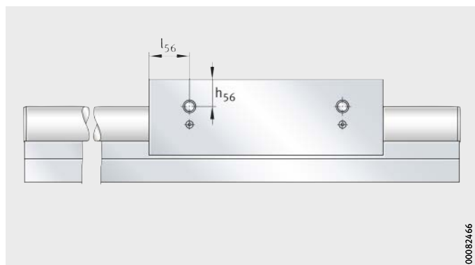
Figure 9 Lubrication points
