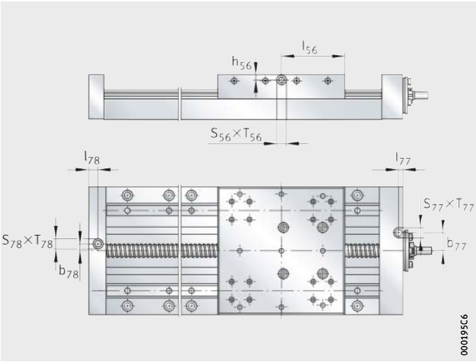
Figure 6 Lubrication points
