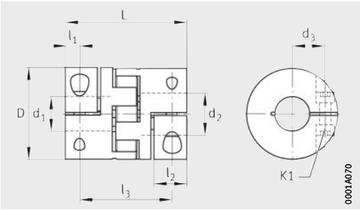
Elastomer coupling
