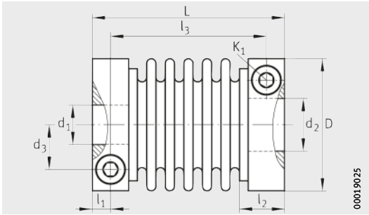
Coupling KUP
