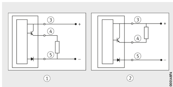
Figure 6 Connection diagram
