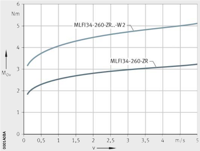
MLFI34.-ZR MLFI34.-ZR..W2 v = travel velocity of carriage M_{0v} = idling drive torque Figure 41 Idling drive torque Vertical mounting position
