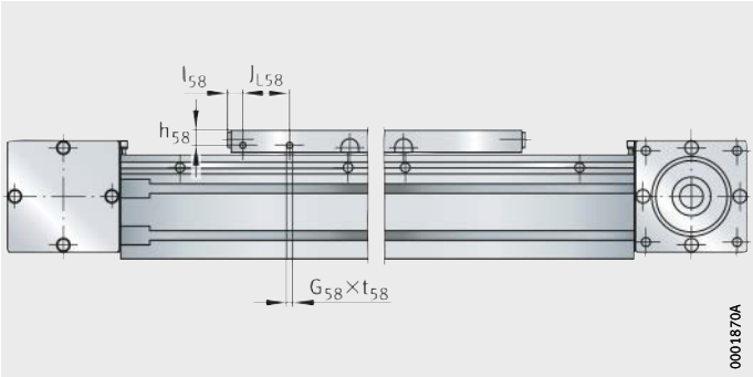
Figure 62 Connectors for switching tags on the carriage
