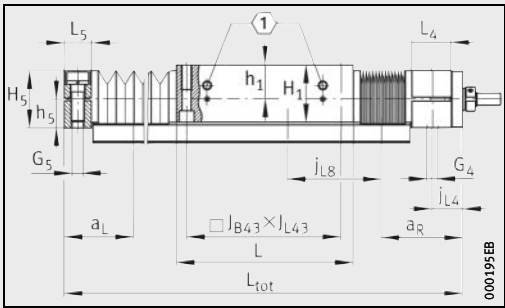
LTS · With bellows (1) 3)
