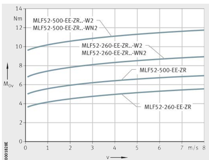
Figure 25 Idling drive torque Vertical mounting position
