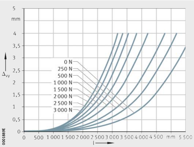
Figure 11 Deflection about the z axis
