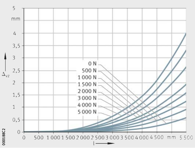
Figure 5 Deflection about the y axis
