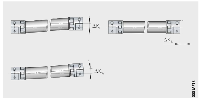
Figure 7 Shaft offset
