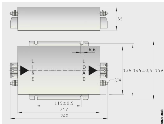
Figure 24 Dimensions
