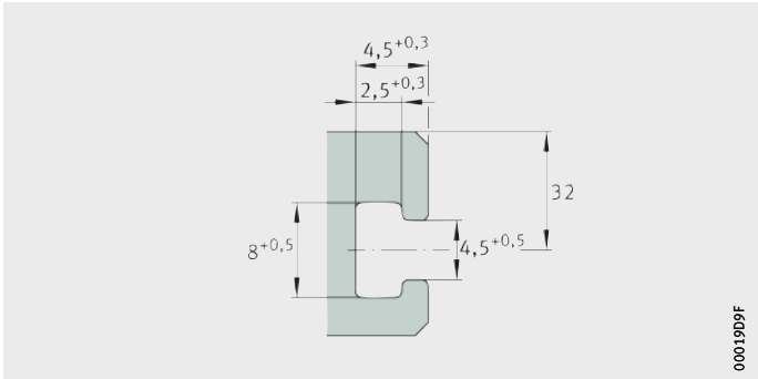
Figure 27 T-slot size in shaft support block
