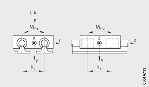
Mounting geometry of linear ball bearings
