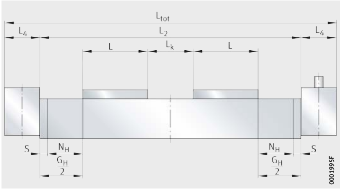
Figure 4 Length parameters
