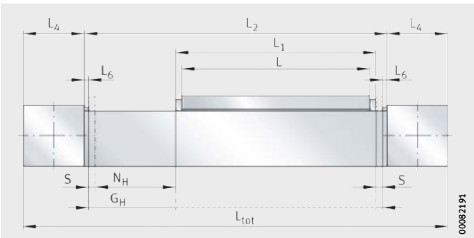
Figure 35 Length parameters for one carriage unit
