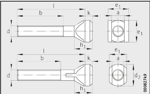
T-bolts in accordance with DIN 787 (both head designs possible)
