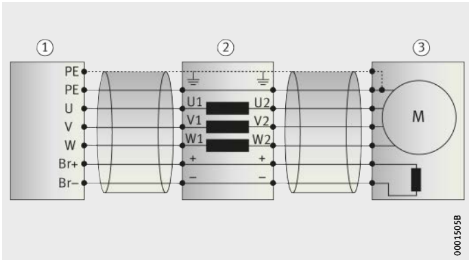
Figure 6 Assignment scheme
