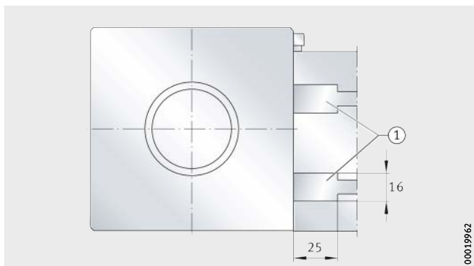
Figure 33 Filling opening in support rail
