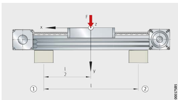
Figure 7 Deflection about the z axis
