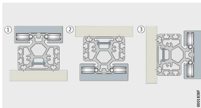
Figure 37 Mounting positions
