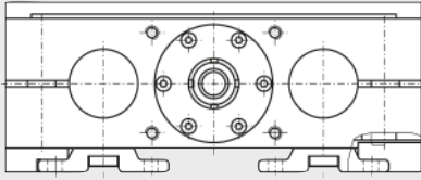
LTS40 and LTS50 · With bellows
