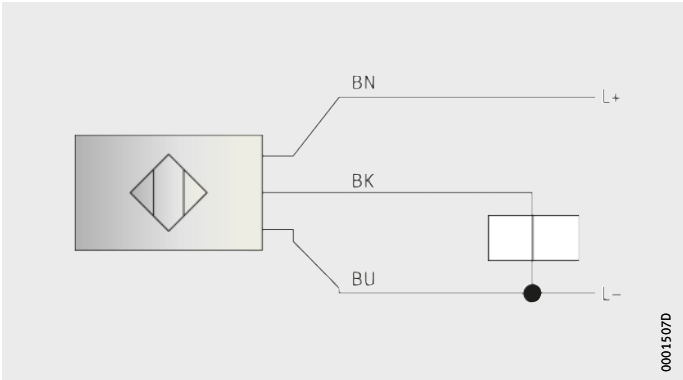
Figure 16 Assignment scheme
