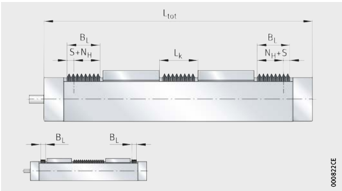
Figure 4 Effective length calculation
