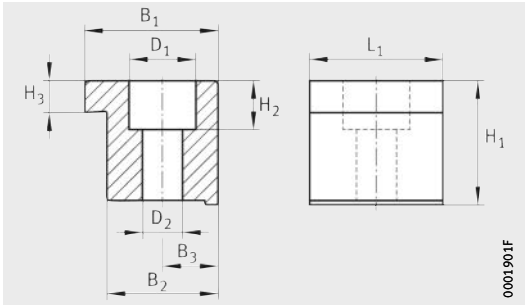
Clamping lugs SPPR
