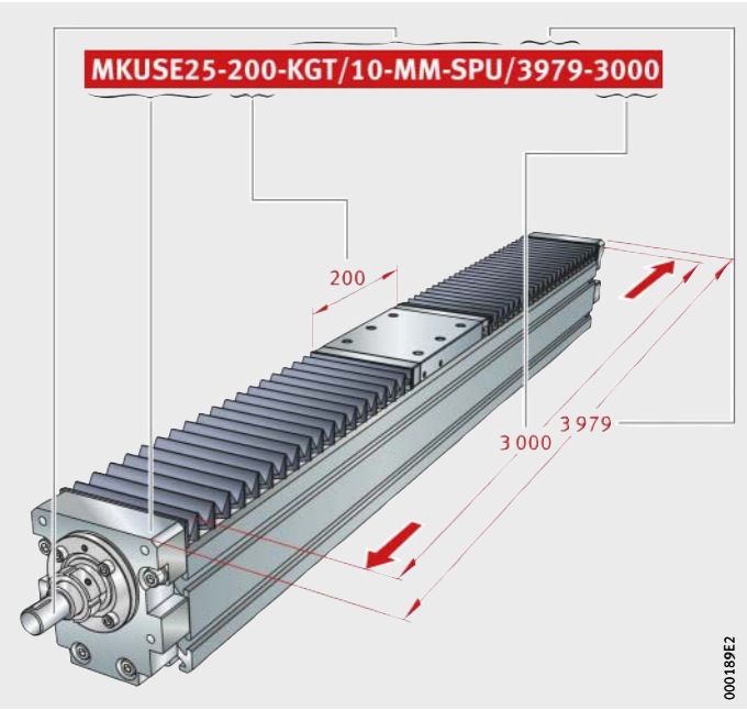
Figure 53 Ordering designation
