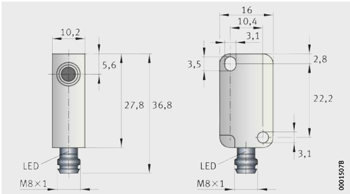
Figure 8 Dimensions
