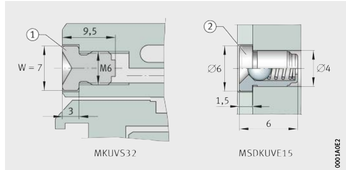
Figure 38 Lubrication nipples
