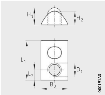
MU..-POS · Positionable T-nut
