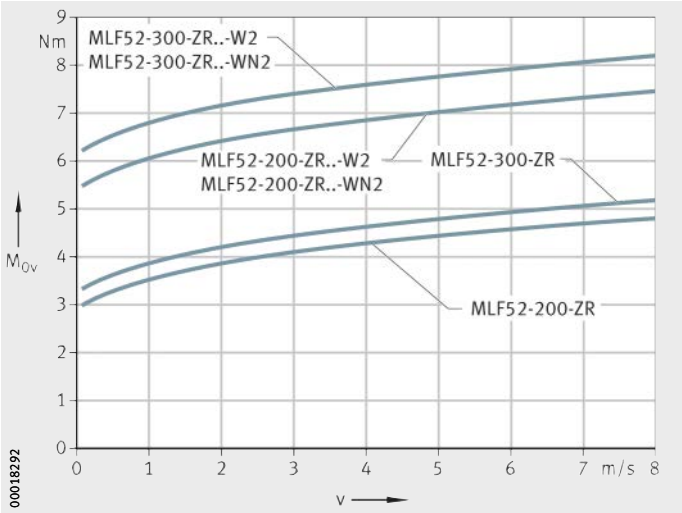
MLF52...-ZR MLF52...-ZR...-W2 MLF52...-ZR...-WN2 v = travel velocity of carriage M_{Ov} = idling drive torque Figure 21 Idling drive torque Vertical mounting position
