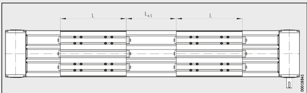
MDKUE...-3ZR-W2-N · Top view 1)
