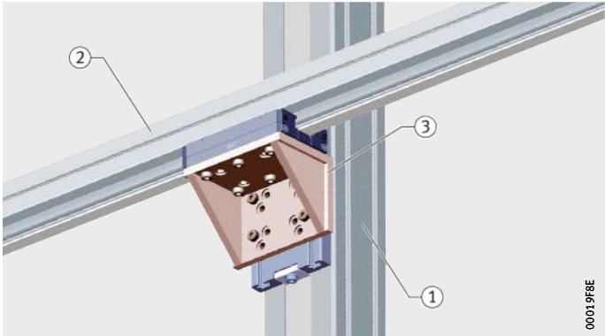
Figure 4 Mounting arrangement 1 Allocation, see table
