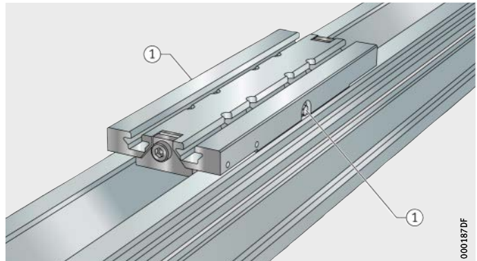
Figure 41 Lubrication points on short carriage unit
