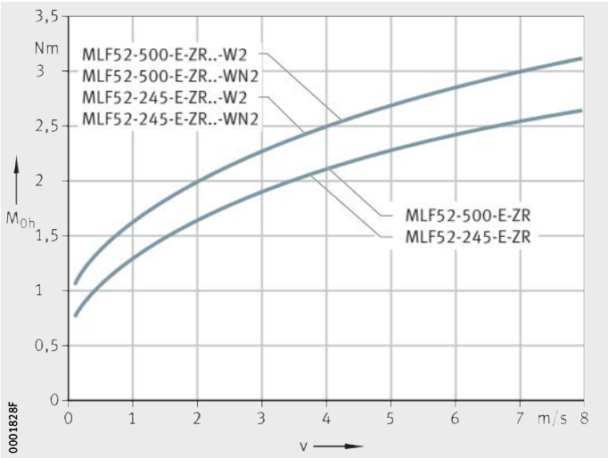
MLF52...-E-ZR MLF52...-E-ZR...-W2 MLF52...-E-ZR...-WN2 v = travel velocity of carriage M_{Oh} = idling drive torque Figure 22 Idling drive torque Horizontal mounting position
