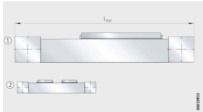
① Basic design ② Second carriage unit (WN2) Figure 34 Basic and additional designs
