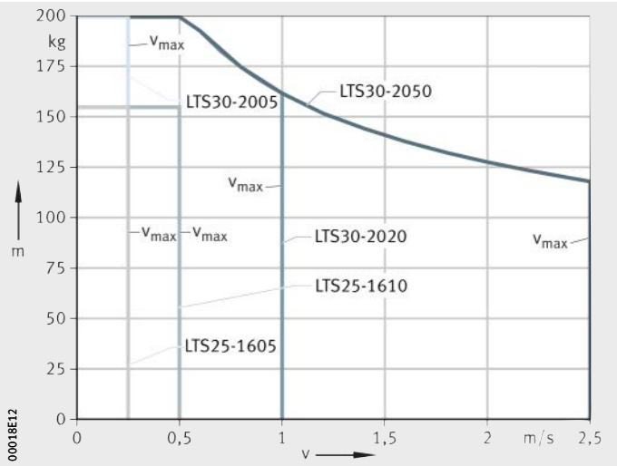
Figure 50 Mass/velocity diagram Horizontal mounting position
