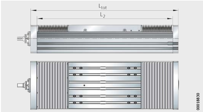
Figure 48 Length tolerances
