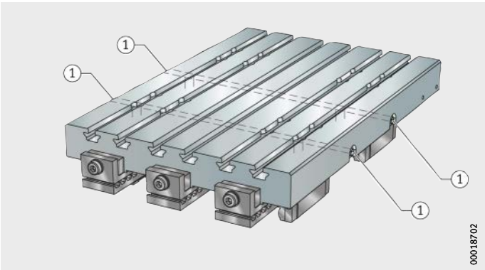
Figure 28 Lubrication ducts in the carriage unit
