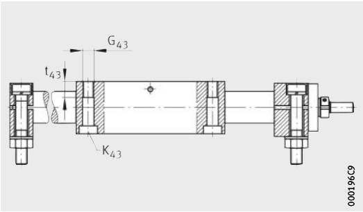
LTE...-A-TGT, LTE...-A-KGT Carriage unit · Fixing screws
