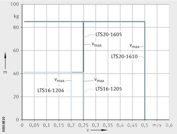
Figure 48 Mass/velocity diagram Horizontal mounting position
