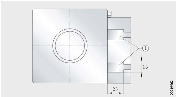
① Filling opening Figure 13 Filling opening in support rail
