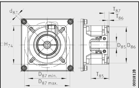
Planetary gearbox with reduction ratio i = 8 with drive flange 2)
