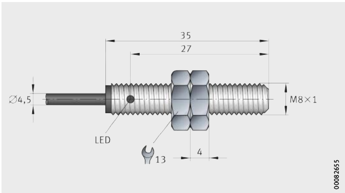
Figure 10 Dimensions
