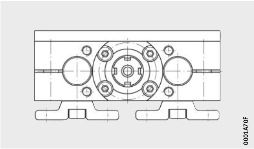
LTS16 · Without bellows
