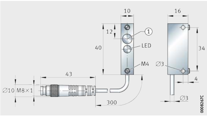
Figure 15 Dimensions of inductive limit switches
