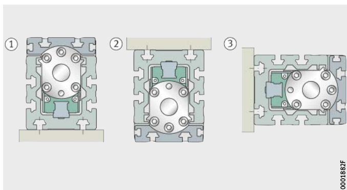
Figure 47 Mounting positions
