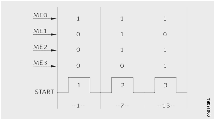
Figure 30 Positional record
