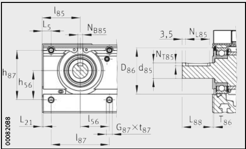
MLFI34-260-ZR · Drive flange, drive shaft
