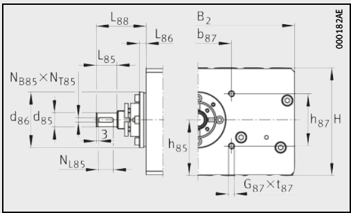
MDKUE...KGT/...N · Drive flange, drive shaft
