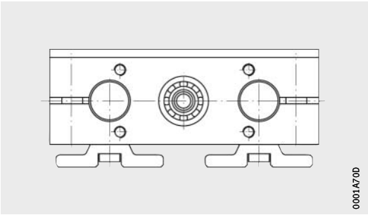
LTS16 to LTS30 · Without bellows
