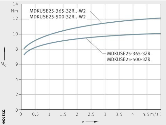
MDKUSE25...3ZR MDKUSE25...3ZR...W2 v = travel velocity of carriage unit M_{0h} = idling drive torque Figure 20 Idling drive torque Horizontal mounting position
