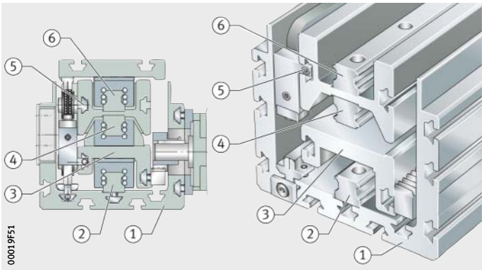
Figure 3 Telescopic support rail unit
