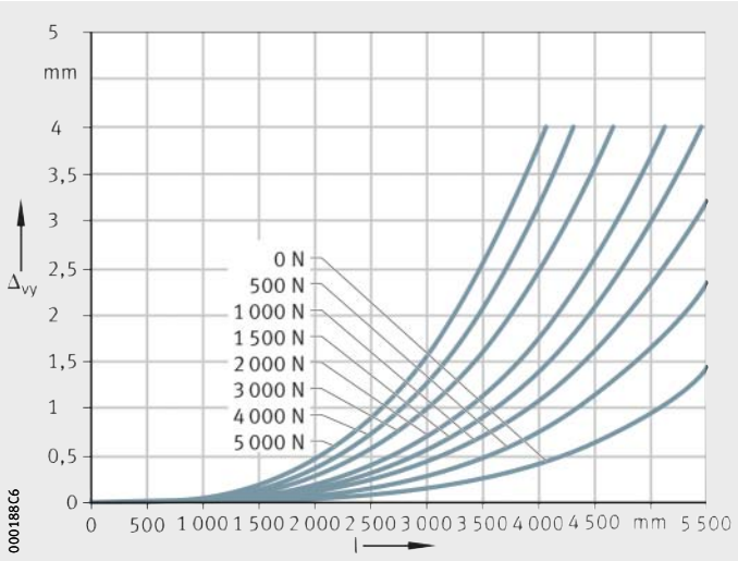
Figure 7 Deflection about the z axis
