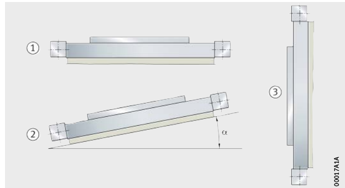
Figure 64 Mounting positions
