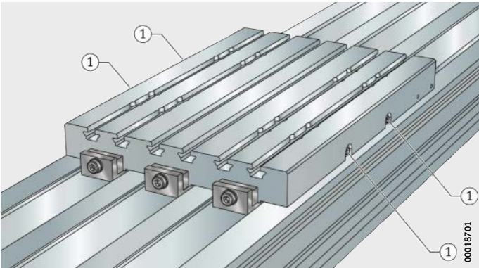
Figure 27 Lubrication points
