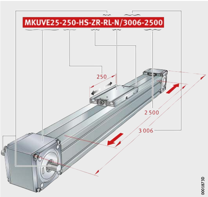
Figure 54 Ordering designation
