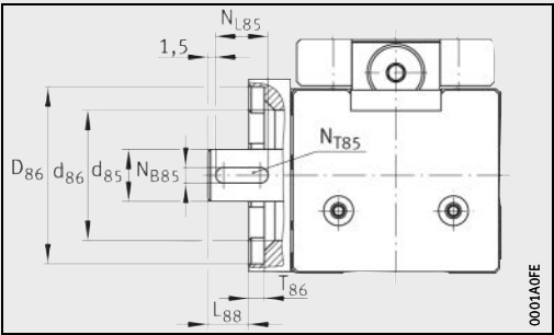
MLFI20...-ZR · Drive flange, drive shaft
