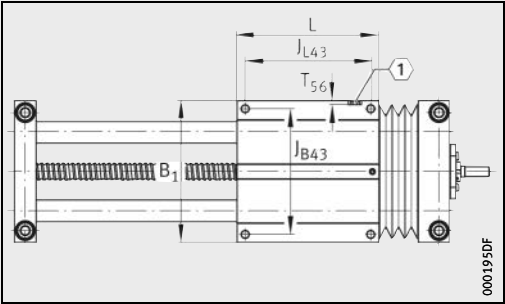
LTE · Top view (1) 2)
