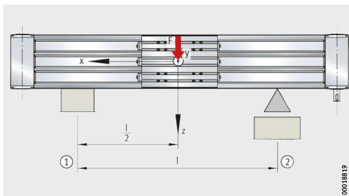
Figure 8 Deflection about the y axis
