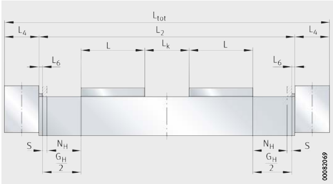
Figure 10 Length features of the actuator Two carriages without bellows
