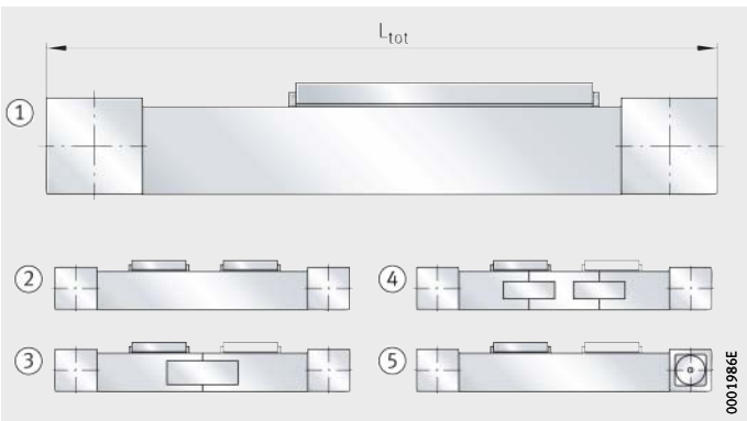
Figure 29 Basic and additional designs Values for mass calculation
