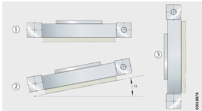
Figure 49 Mounting positions
