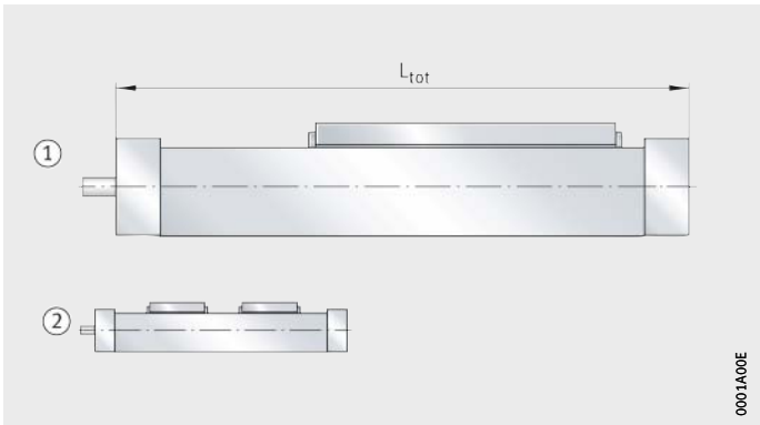
Figure 23 Basic and additional designs
