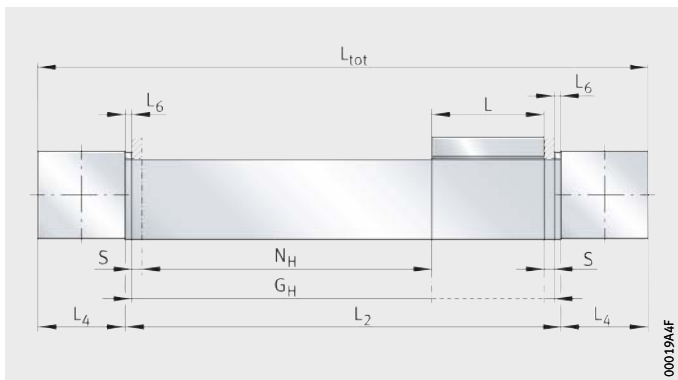
Figure 26 Length parameters for one carriage
