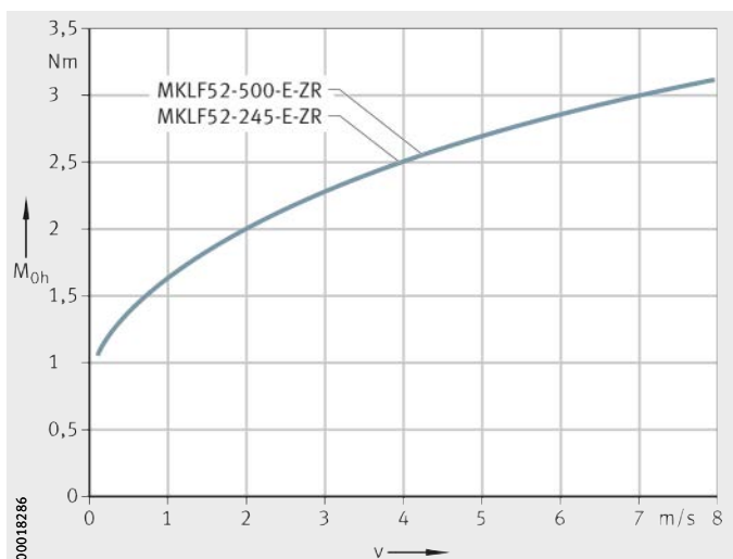
Figure 6 Idling drive torque Horizontal mounting position
