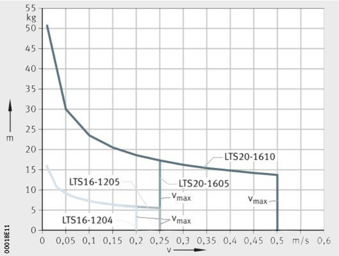
Figure 49 Mass/velocity diagram Vertical mounting position
