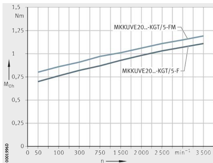
Figure 1 Idling drive torque Horizontal mounting position
