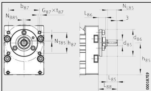
MKKUBE20-200-KGT/5-N · Drive flange, drive shaft
