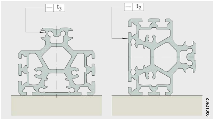
t_2, t_3 = straightness tolerance Figure 40 Measurement method for straightness tolerances
