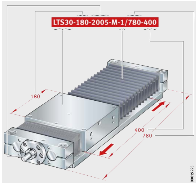
Figure 16 Ordering designation
