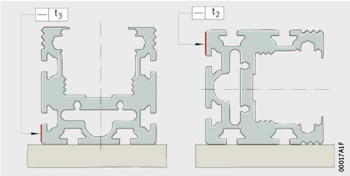
Figure 68 Measurement method for straightness tolerances
