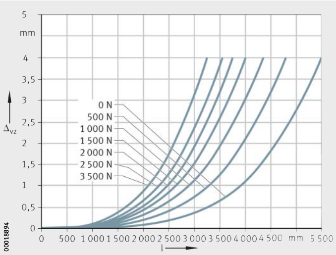
Figure 17 Deflection about the y axis
