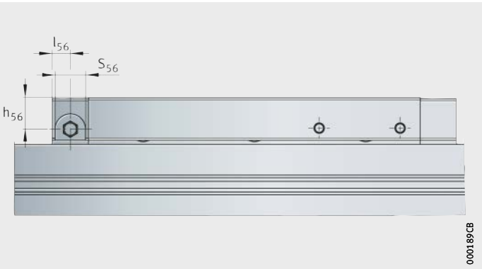
Figure 39 Lubrication points
