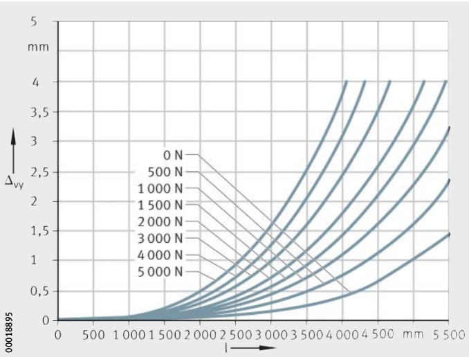
Figure 16 Deflection about the z axis
