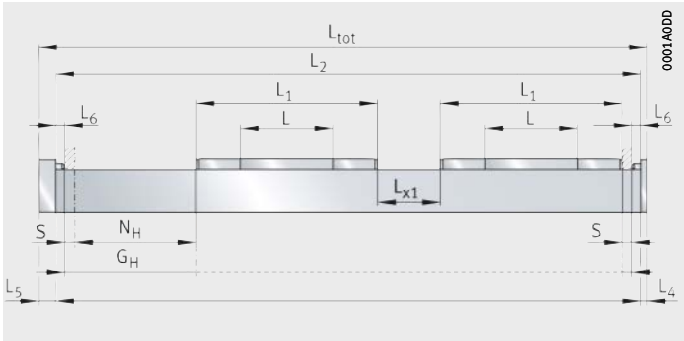
Figure 33 Length parameters for two carriage units
