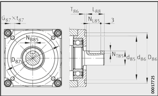
MKLF..ZR · Drive flange, drive shaft
