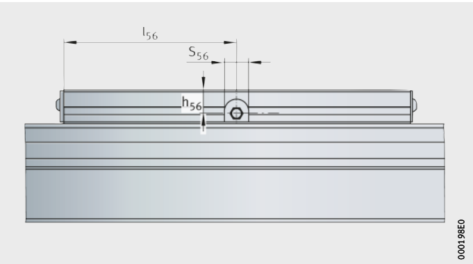
Figure 38 Lubrication points
