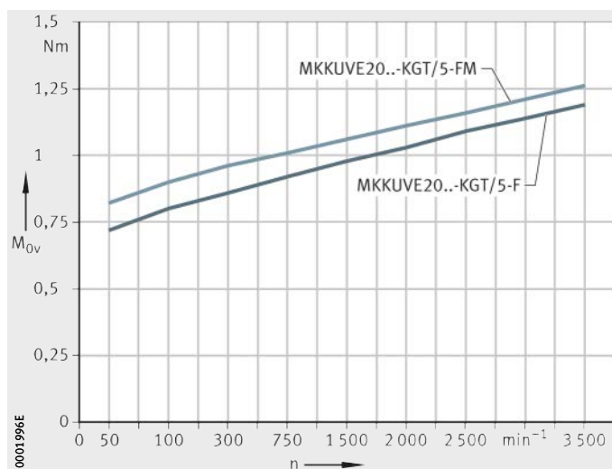
Figure 2 Idling drive torque Vertical mounting position
