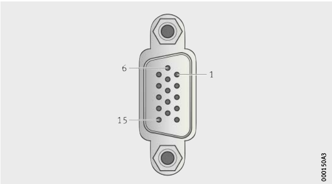
Figure 8 Plug X12
