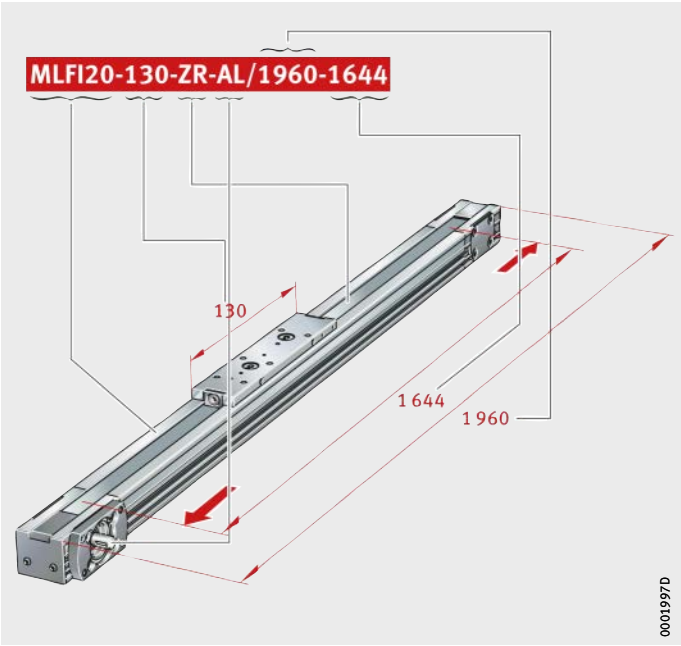
Figure 70 Ordering designation
