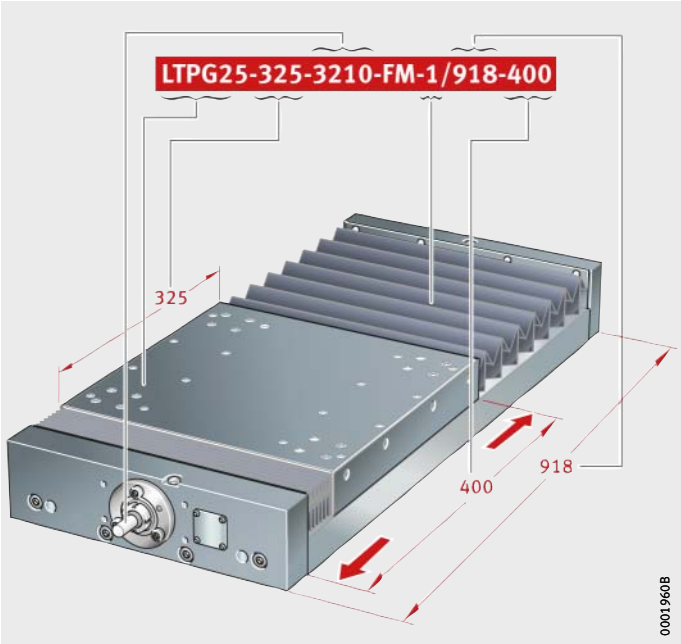
Figure 15 Ordering designation
