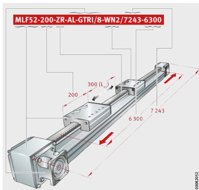
Figure 42 Ordering designation
