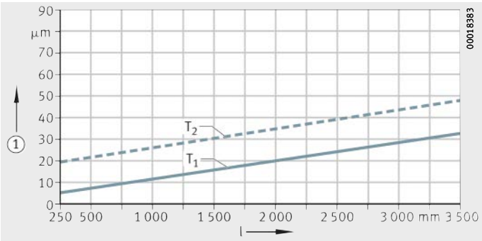
Figure 13 Accuracy values
