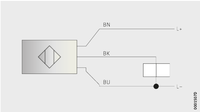
Figure 6 Assignment scheme
