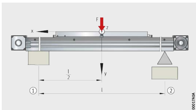
Figure 8 Deflection about the z axis
