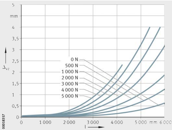
Figure 7 Deflection about the y axis
