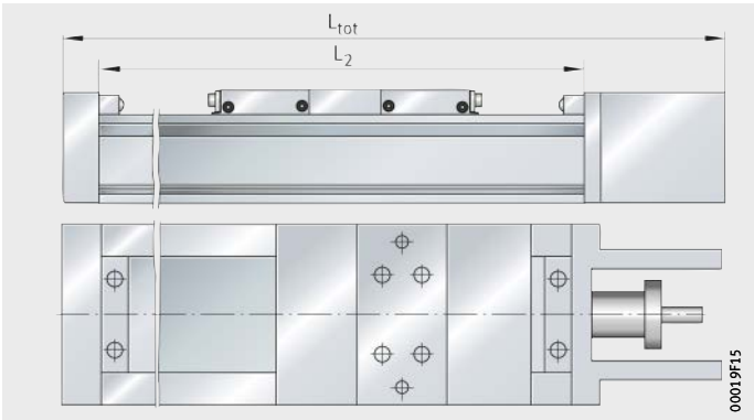
Figure 44 Length tolerances
