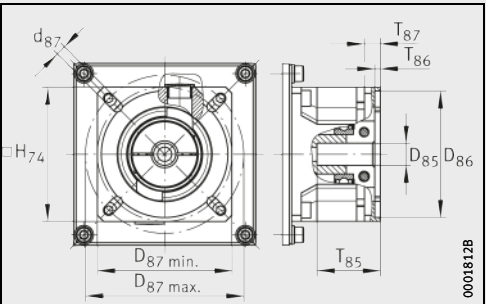
Planetary gearbox with reduction ratio i = 8 with drive flange
