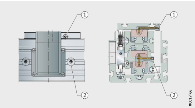
Figure 13 Lubrication points on telescopic actuator
