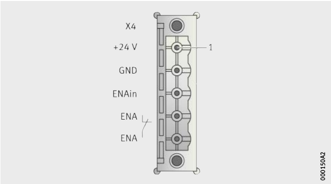
Figure 3 Plug X4
