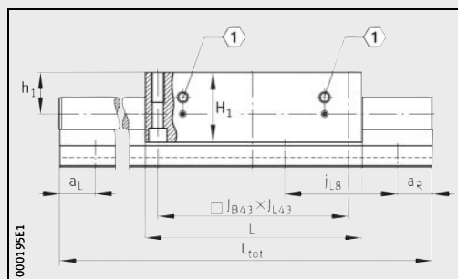
LTS · Without bellows
