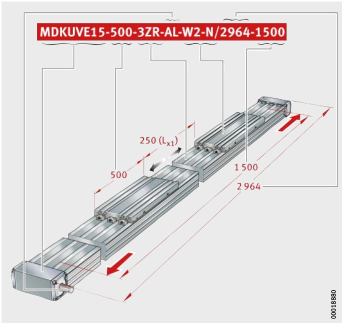
Figure 34 Ordering designation
