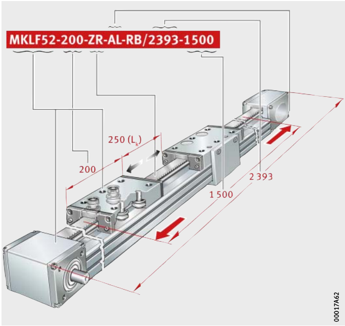
Figure 14 Ordering designation
