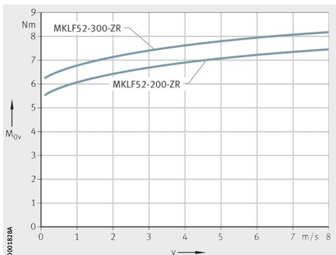
Figure 5 Idling drive torque Vertical mounting position
