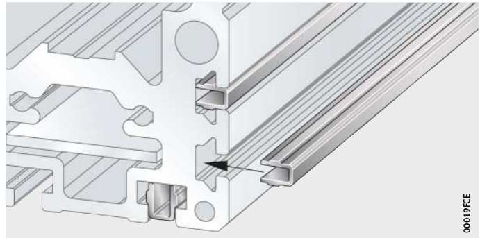
Figure 7 Slot closing strip NAD
