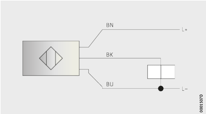
Figure 3 Assignment scheme
