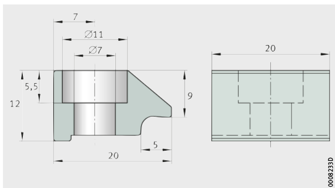
Figure 10 Dimensions of clamping lug
