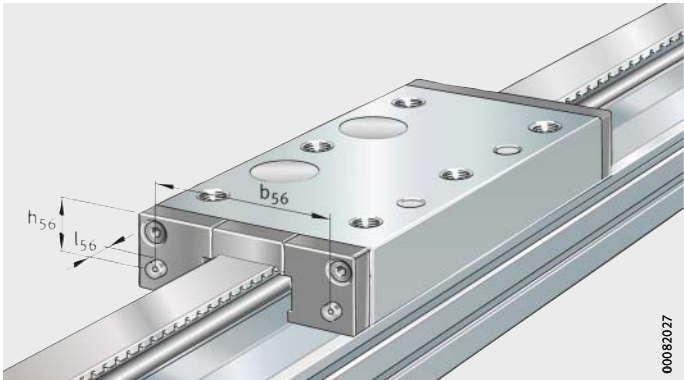
Figure 31 Lubrication points
