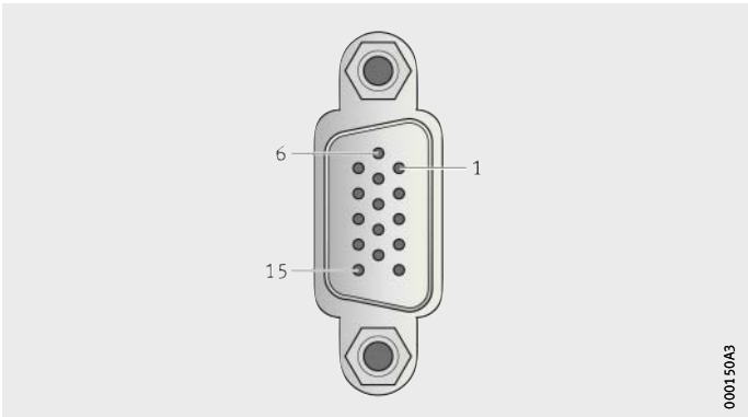
Figure 9 Plug X22
