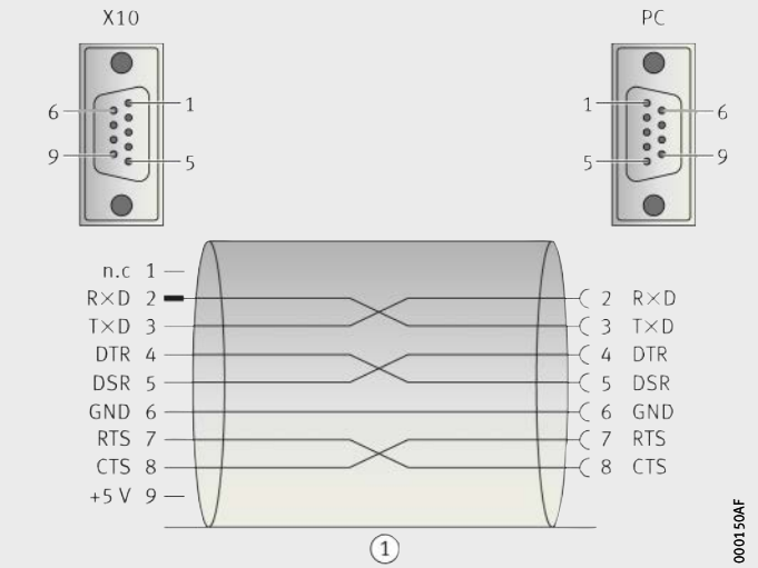
Figure 26 Wiring plan
