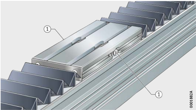
Figure 6 Lubrication points
