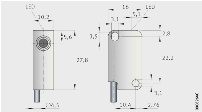
Figure 5 Dimensions
