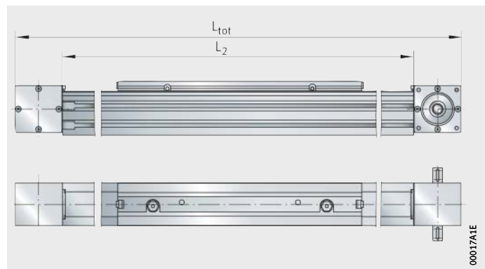
Figure 67 Length tolerances
