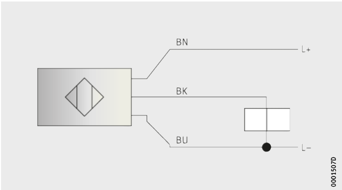
Figure 11 Assignment scheme
