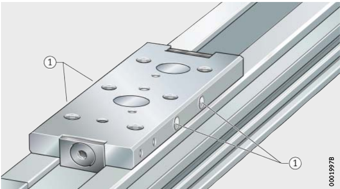
Figure 56 Lubrication points
