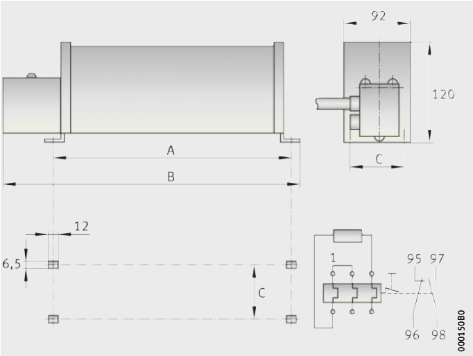
Figure 20 Dimensions
