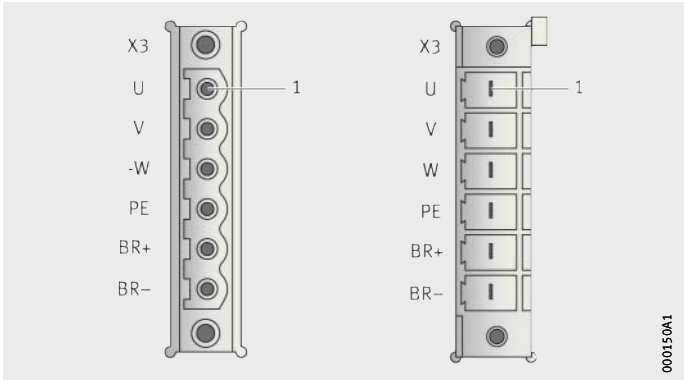
Figure 4 Plug X3
