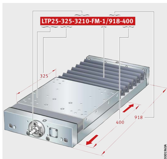
Figure 14 Ordering designation
