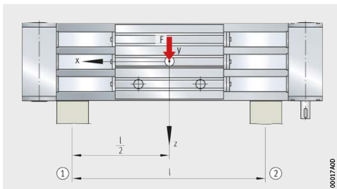
Figure 11 Deflection about the y axis
