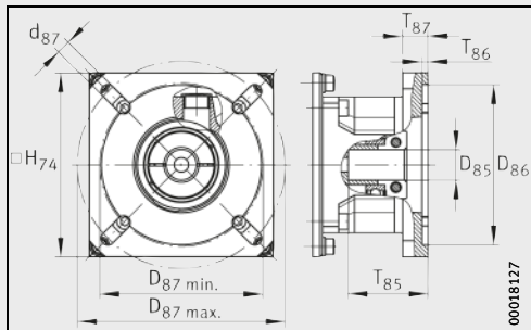
Planetary gearbox with reduction ratio i = 4 with drive flange
