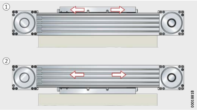
Figure 47 Movable or stationary carriage
