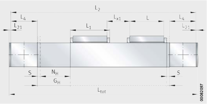
Figure 51 Length parameters for two carriages
