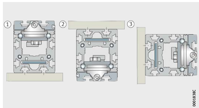
Figure 65 Mounting positions
