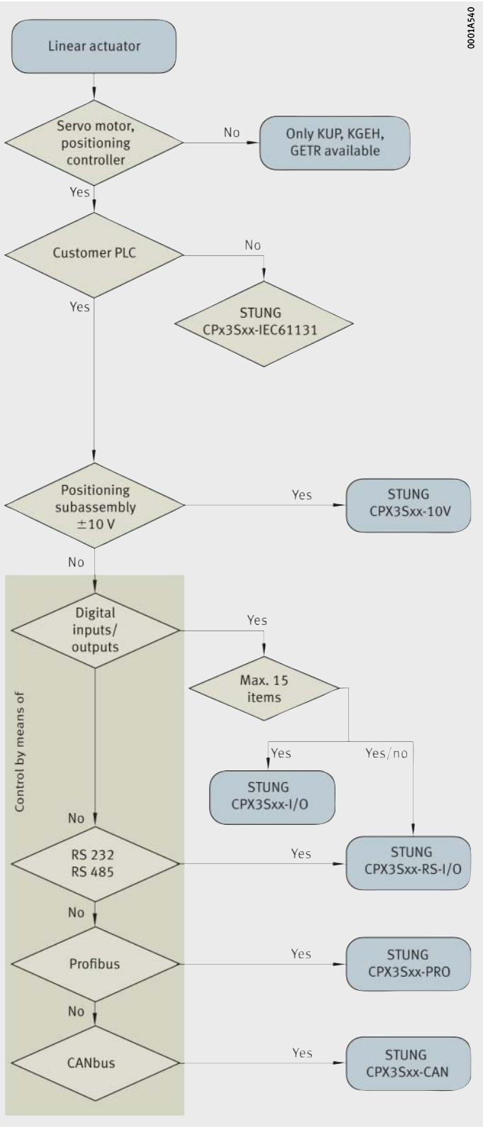
Figure 1 Flow chart
