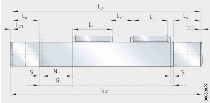
Figure 36 Length parameters for two carriage units
