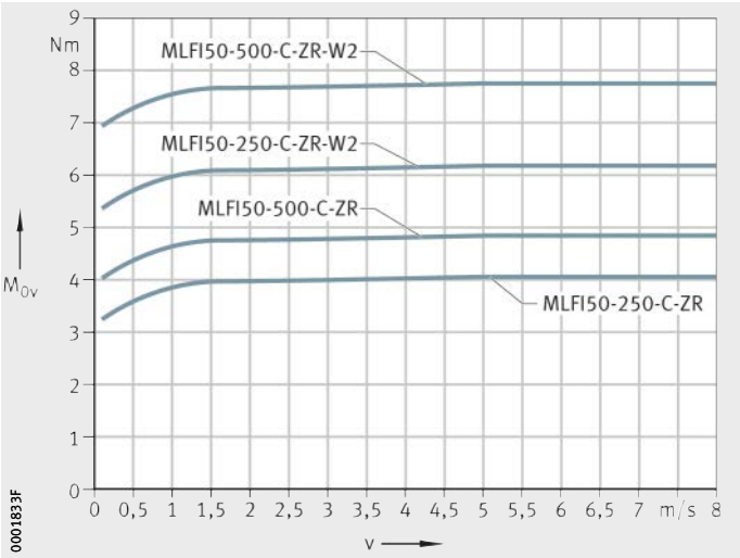
MLFI50.-C-ZR MLFI50.-C-ZR..W2 v = travel velocity of carriage M_{0v} = idling drive torque Figure 43 Idling drive torque Vertical mounting position
