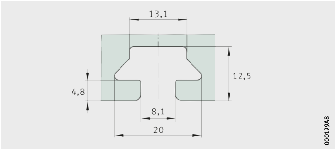
MKLF Figure 12 Dimensions of T-slots
