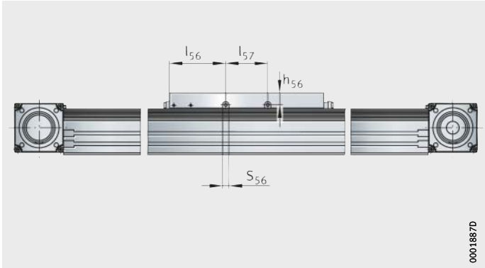
Figure 29 Lubrication points
