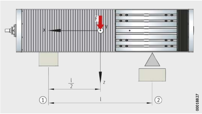
Figure 5 Deflection about the y axis
