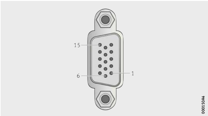
Figure 5 Plug X13
