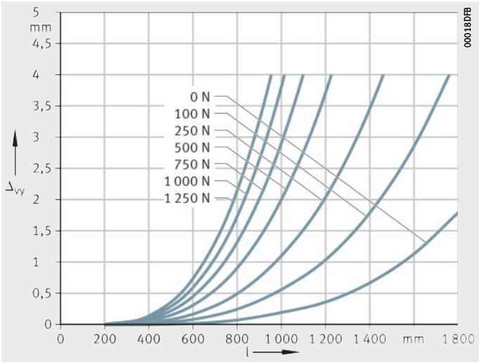
LTE20 Locating/non-locating bearing arrangement \Delta_{vy} = deflection l = support spacing Figure 11 Deflection about the z axis
