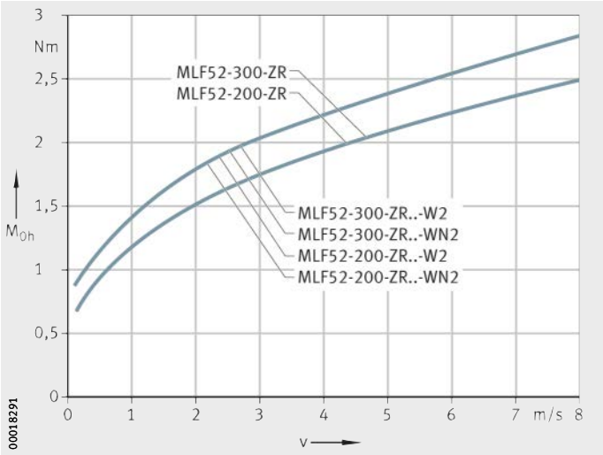
MLF52...-ZR MLF52...-ZR...-W2 MLF52...-ZR...-WN2 v = travel velocity of carriage M_{Oh} = idling drive torque Figure 20 Idling drive torque Horizontal mounting position
