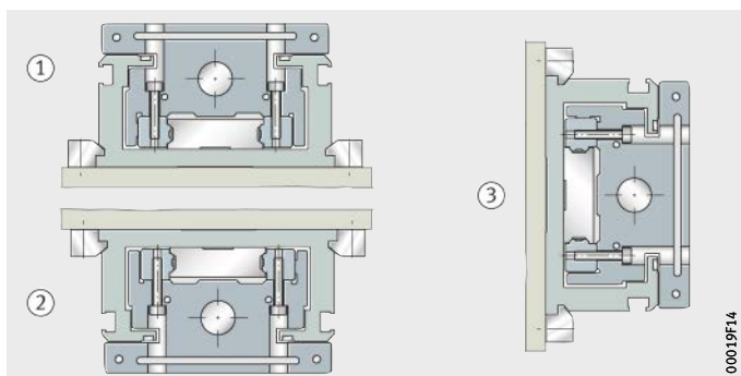
Figure 43 Mounting positions
