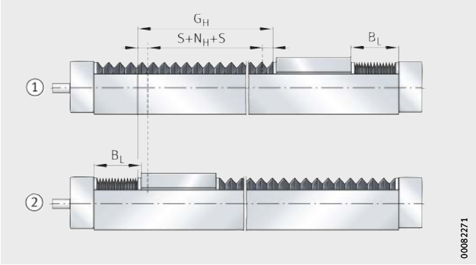
Figure 22 Effective length calculation
