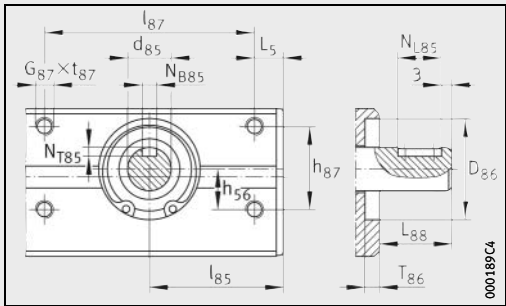
MLFI25...-ZR-N · Drive flange, drive shaft
