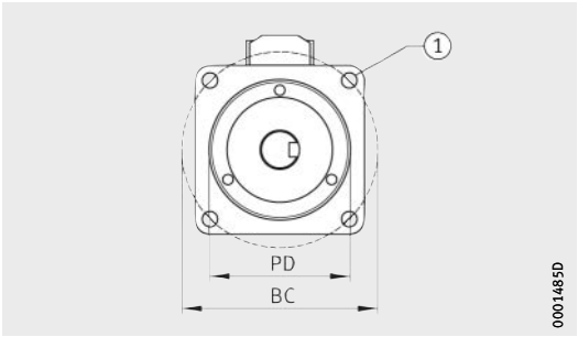
Mounting dimensions for motor adapter plates ① 3)
