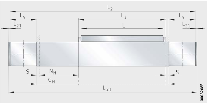
Figure 34 Length parameters for one carriage unit
