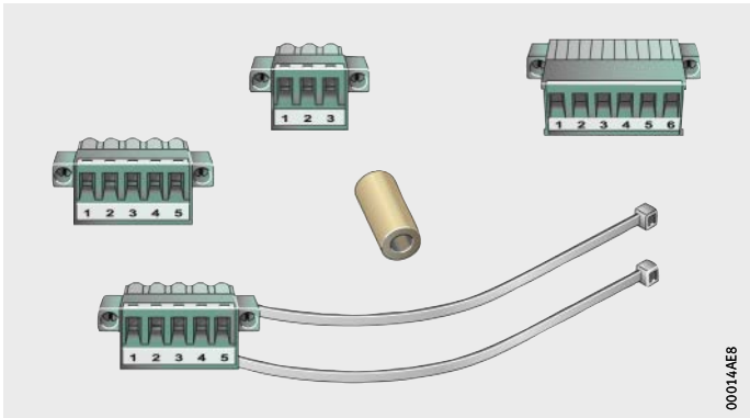
Figure 12 Connector set
