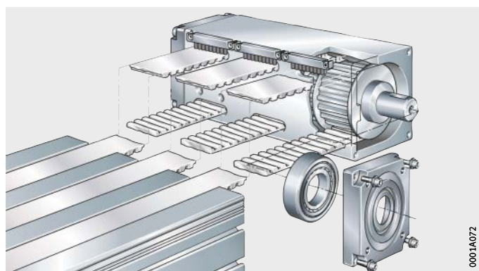
Figure 2 Return unit for triple toothed belt drive
