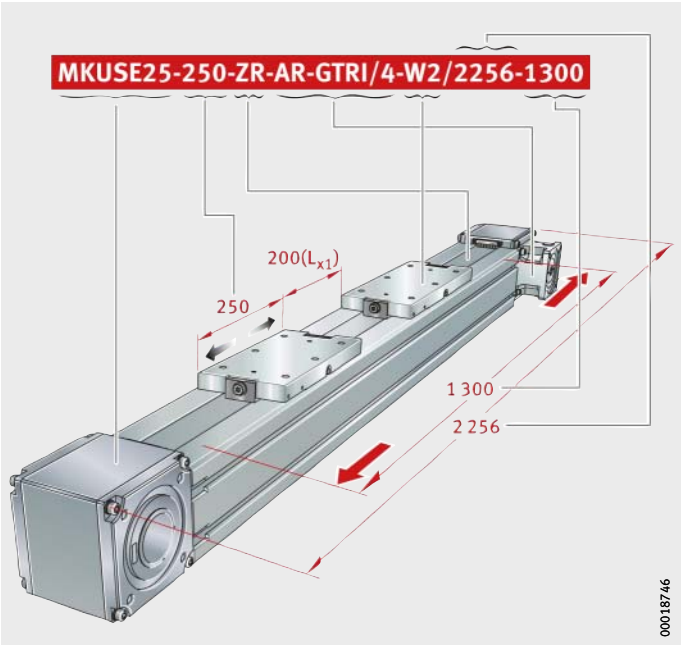
Figure 56 Ordering designation
