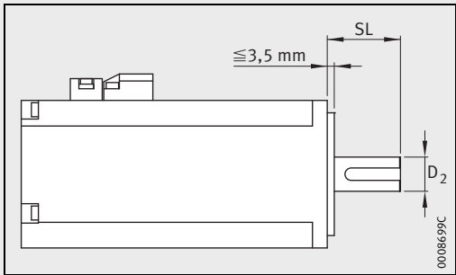
Mounting dimensions for motor adapter plates
