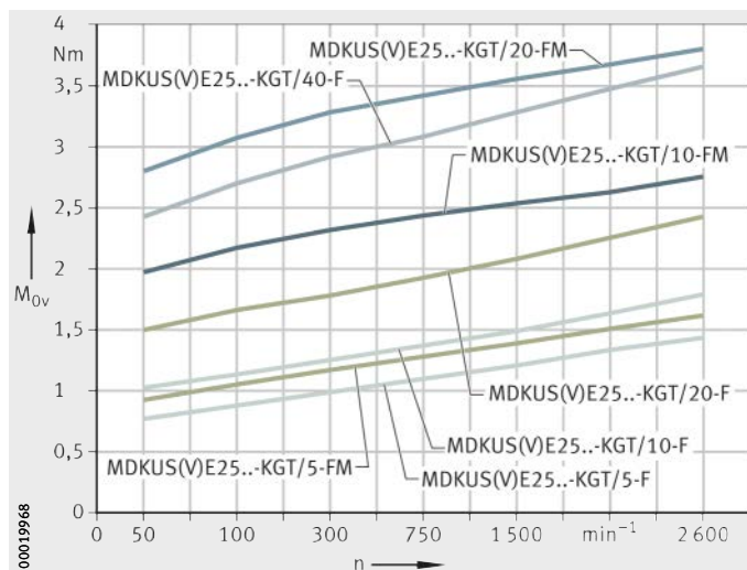
Figure 17 Idling drive torque Vertical mounting position
