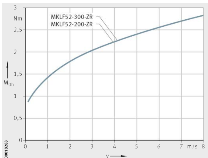
Figure 4 Idling drive torque Horizontal mounting position
