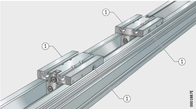
Figure 6 Lubrication points
