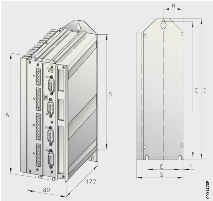
Figure 1 Dimensions
