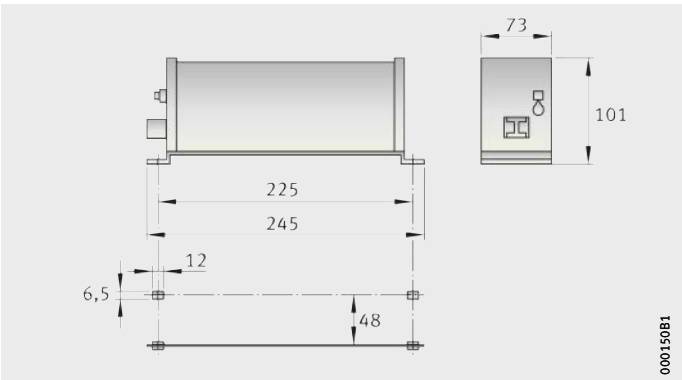
Figure 19 Dimensions
