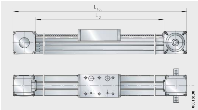
Figure 39 Length tolerances
