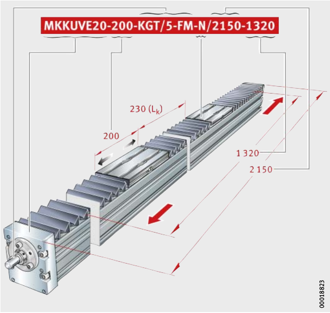
Figure 12 Ordering designation
