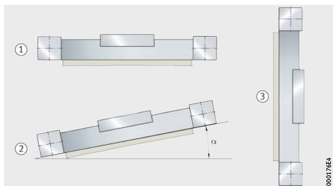
Figure 36 Mounting positions
