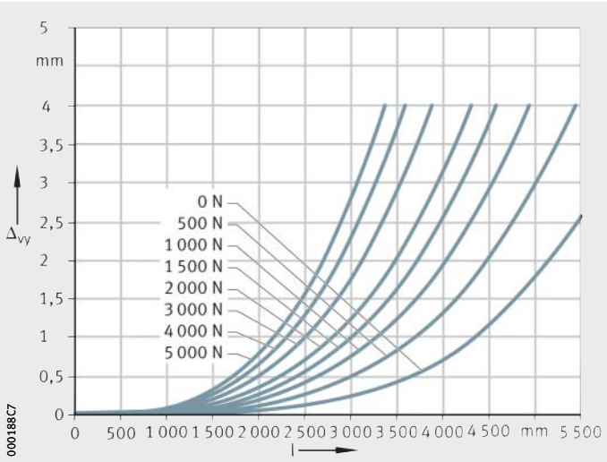
Figure 6 Deflection about the z axis
