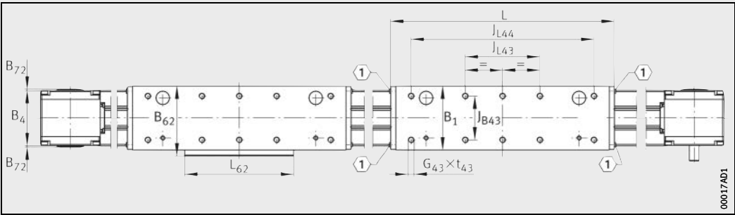
MKLF..ZR · Top view of long carriage (1) 1)
