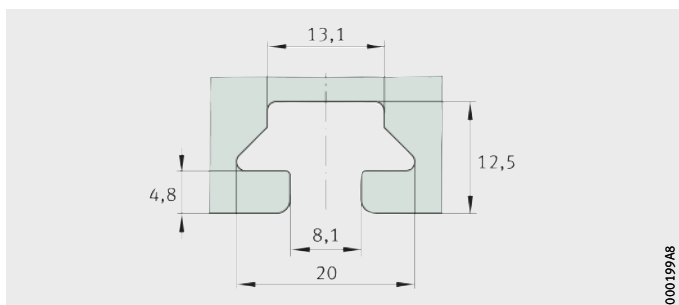
Figure 32 Dimensions of T-slots
