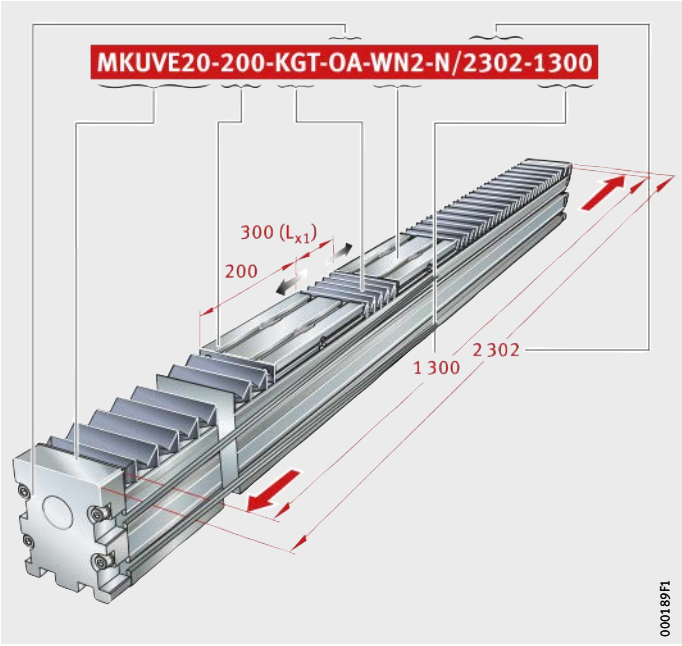
Figure 51 Ordering designation
