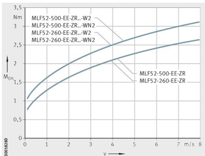
Figure 24 Idling drive torque Horizontal mounting position
