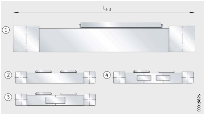
Figure 26 Basic and additional designs
