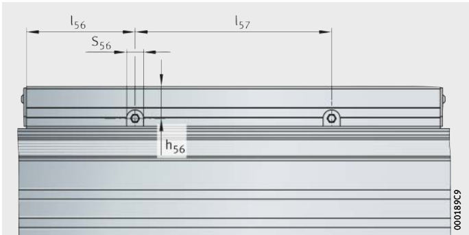
Figure 25 Position of relubrication points
