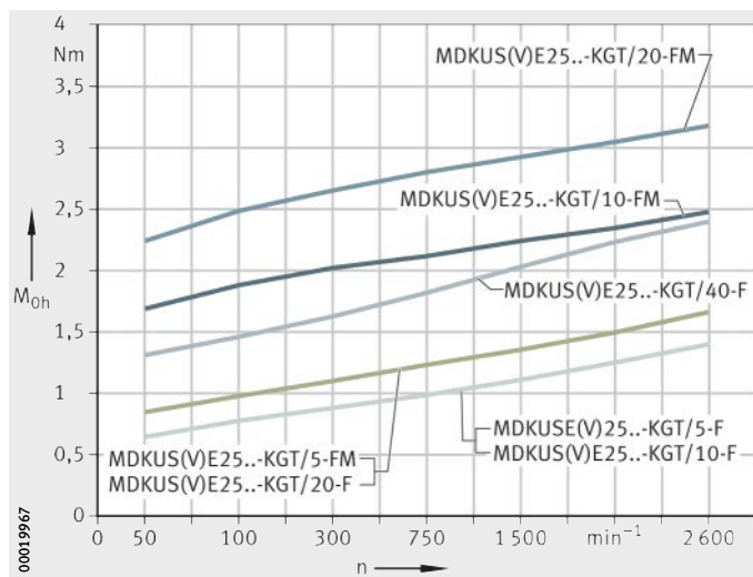
Figure 16 Idling drive torque Horizontal mounting position
