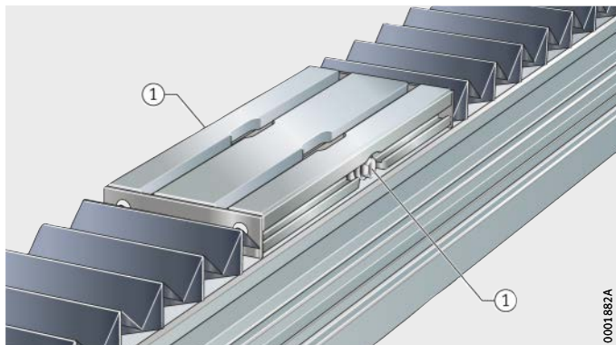
Figure 36 Lubrication points
