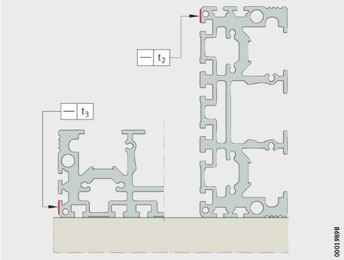
t_2, t_3 = straightness tolerance Figure 33 Measurement method for straightness tolerances
