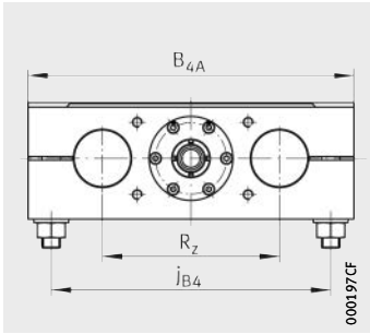
LTE40...-A-TR and LTE50...-A-TR
