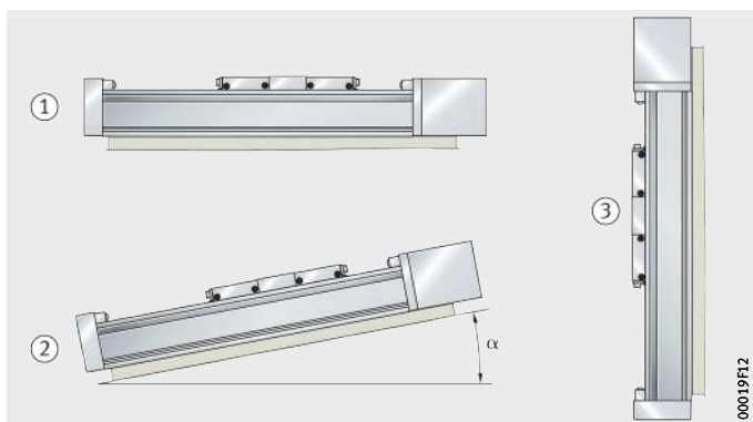
Figure 42 Mounting positions
