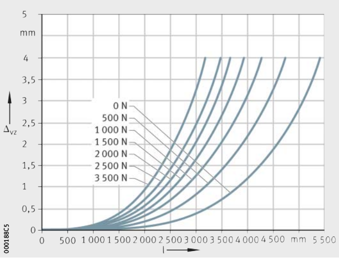
Figure 8 Deflection about the y axis
