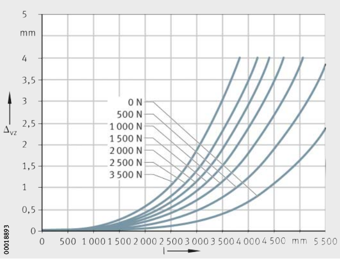
Figure 18 Deflection about the y axis
