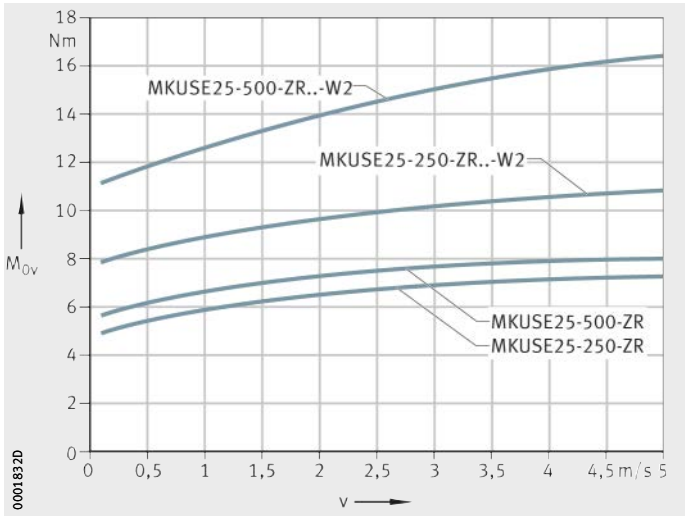
MKUSE25...-ZR MKUSE25...-ZR...W2 v = travel velocity of carriage unit M_{0v} = idling drive torque Figure 33 Idling drive torque Vertical mounting position
