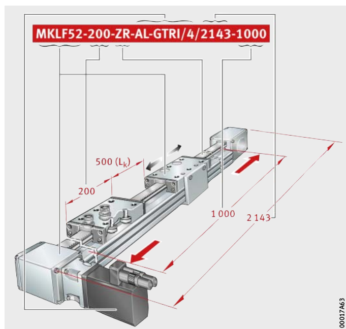
Figure 15 Ordering designation
