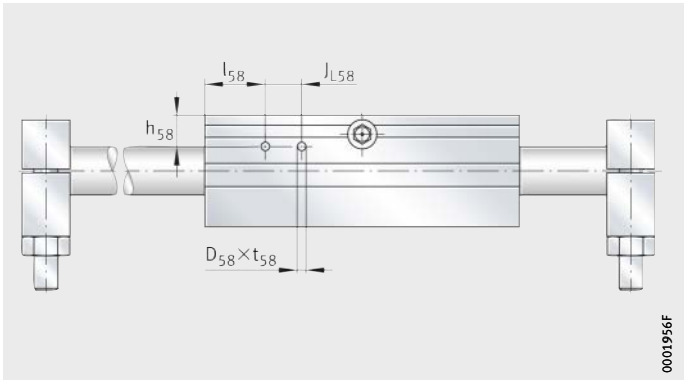
Figure 28 Connectors for switching tags on actuator LTE20-A-OA
