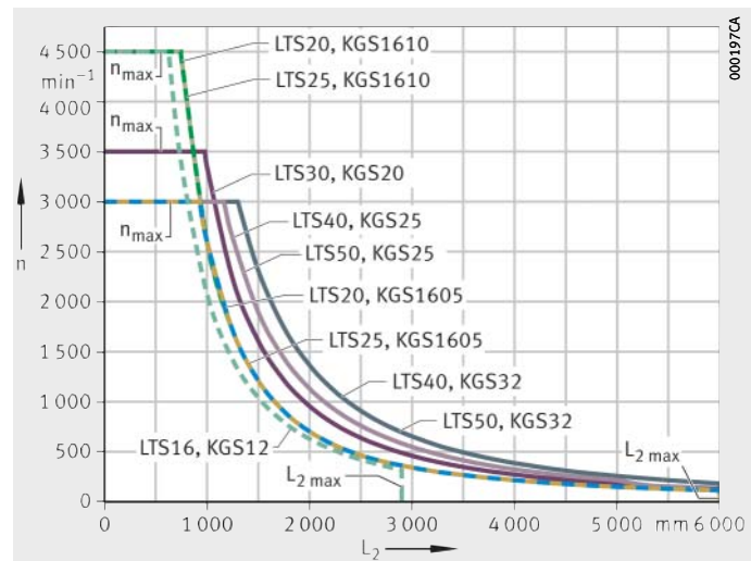
Figure 11 Maximum permissible spindle speed without spindle supports
