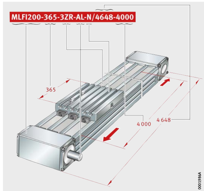
Figure 71 Ordering designation
