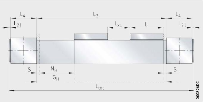
Figure 50 Length parameters for two carriages
