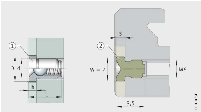
Figure 12 Lubrication nipples
