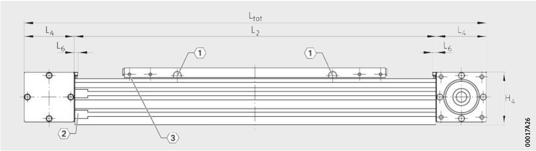
MLFI50-500-C-ZR-N ①, ②, ③ 2)
