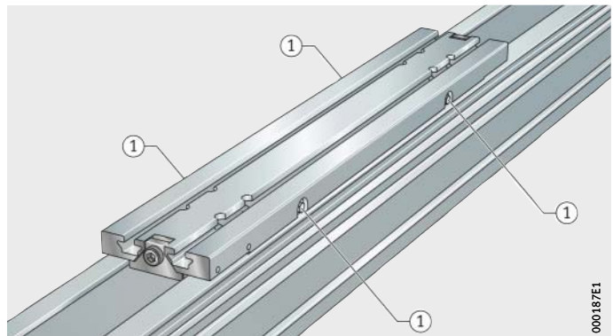
Figure 42 Lubrication points on long carriage unit
