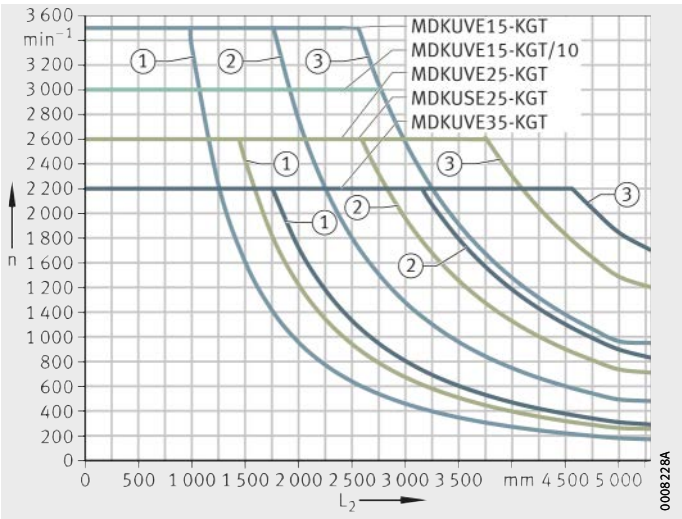
Figure 28 Maximum permissible spindle speed
