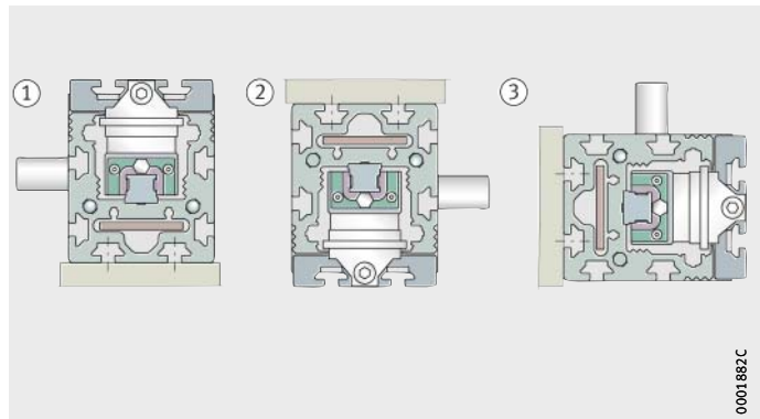
Figure 48 Mounting positions
