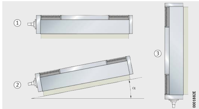
Figure 46 Mounting positions
