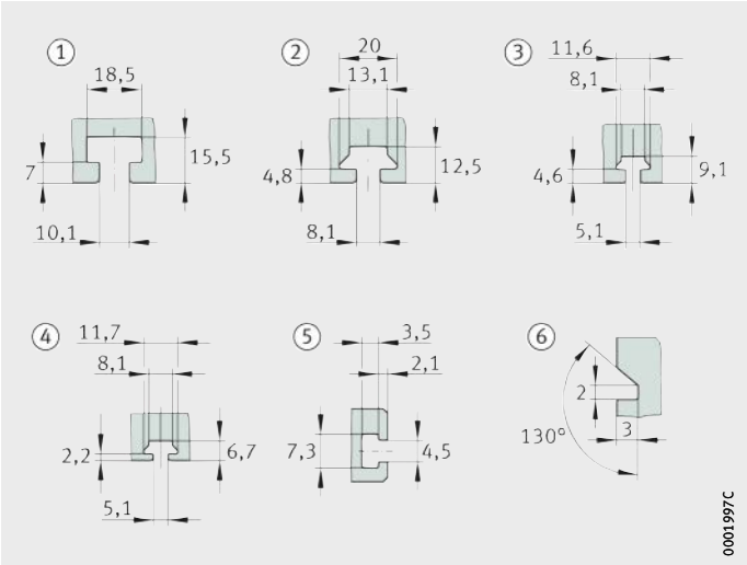
Figure 60 Sizes of T-slots in support rail and carriage
