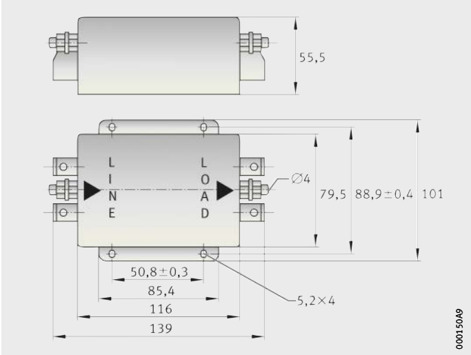
Figure 22 Dimensions
