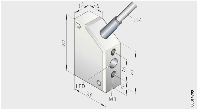
Figure 1 NS-INSOR52-PNP-OEFFNER
