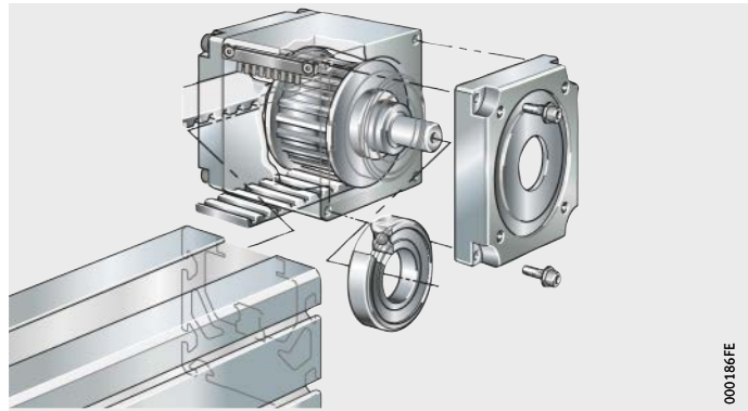
Figure 3 Return unit
