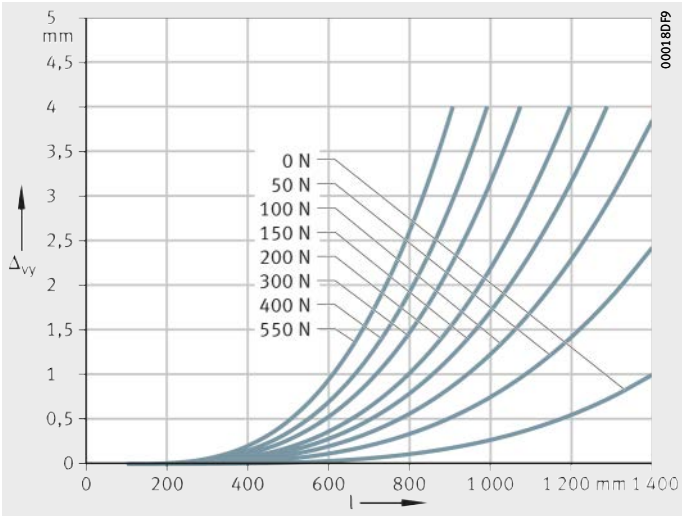
LTE16 Locating/non-locating bearing arrangement \Delta_{vy} = deflection l = support spacing Figure 9 Deflection about the z axis
