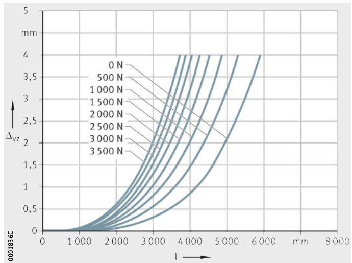
Figure 20 Deflection about the y axis
