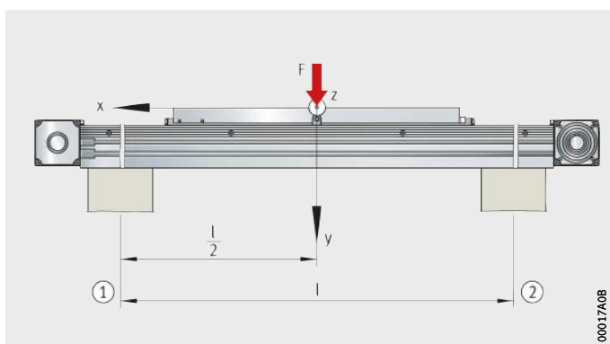
Figure 9 Deflection about the z axis
