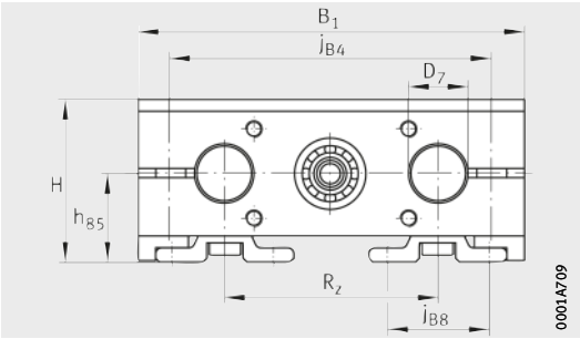
LTS16 to LTS30 · With bellows
