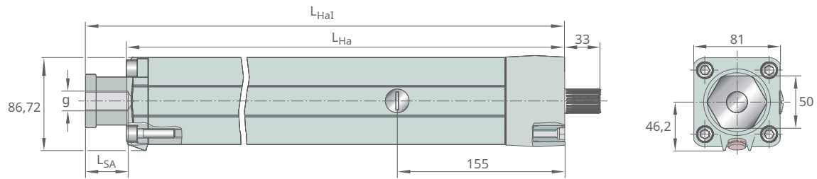
5 Dimensions with female thread on push tube
