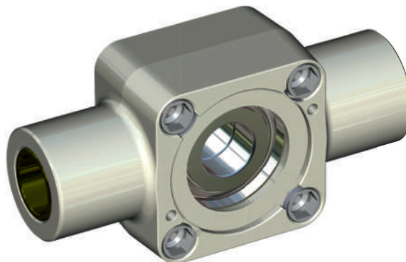
☞18 Bearing housing with female trunnion mount
