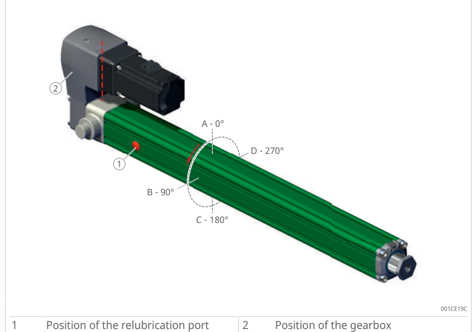
48 Possible orientation of the linear unit
