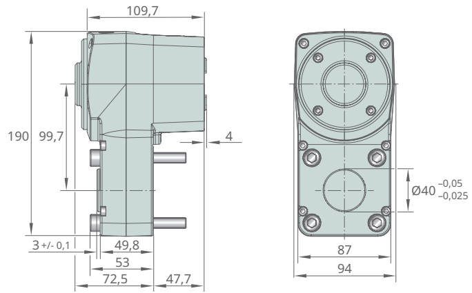
32 Dimensions for 2-stage parallel gearbox
