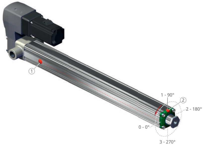
52 Possible orientation of the front cover with vent plug
