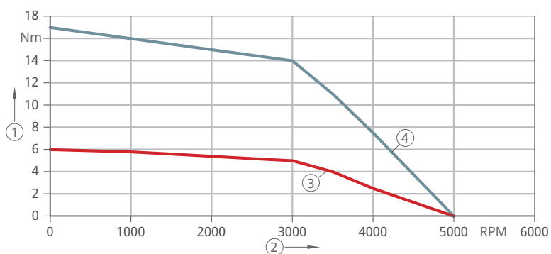
43 Motor speed and motor torque for 1.5 kW motor
