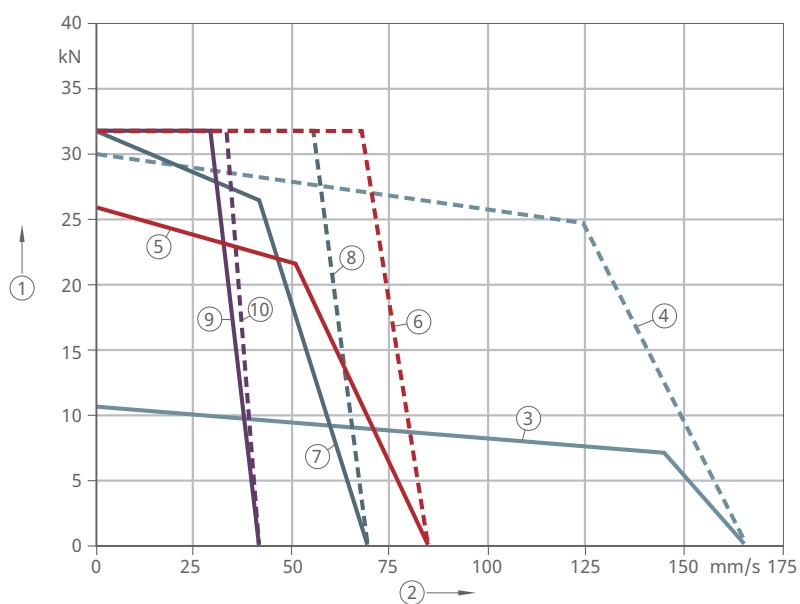
44 Speed-load diagram for 1.5 kW motor
