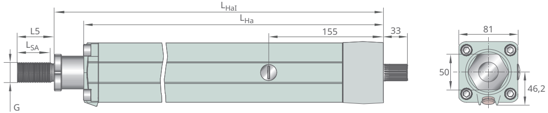
4 Dimensions with male thread on the push tube
