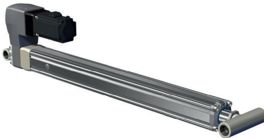
37 EWELLIX-Electric actuator with motor, 2 Nm EM holding brake
