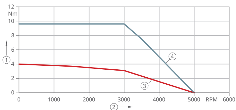
41 Motor speed and motor torque for 1 kW motor
