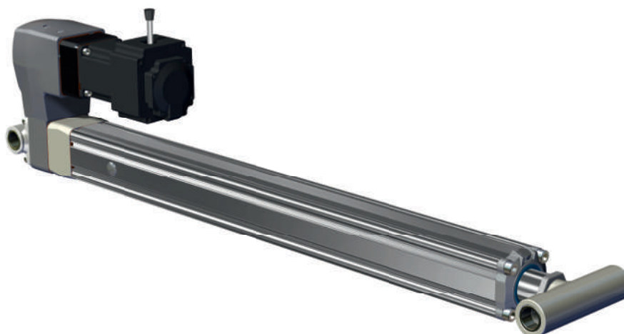
38 EWELLIX-Electric actuator with motor, 10 Nm EM holding brake and manual release
