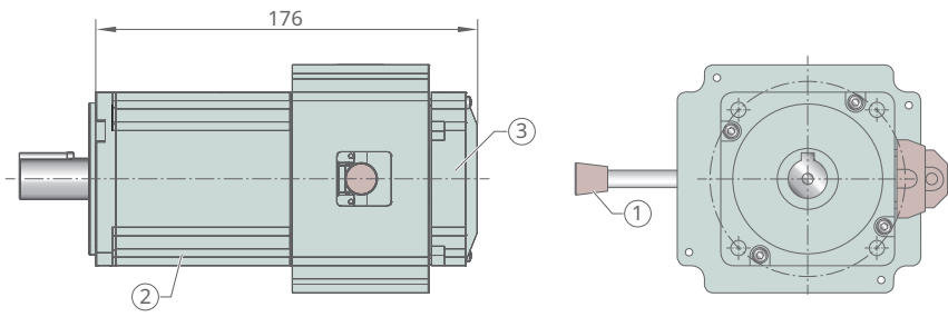
45 Dimensions for 750-W servo motor Fulling FL80SV75
