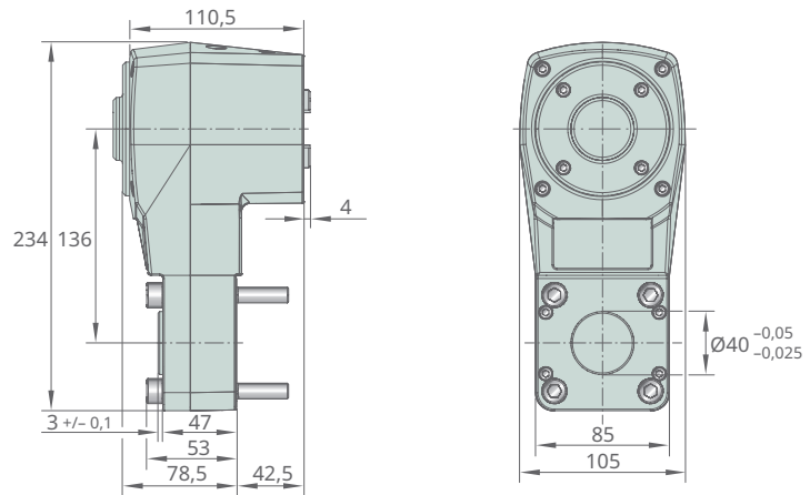
33 Dimensions for 3-stage parallel gearbox
