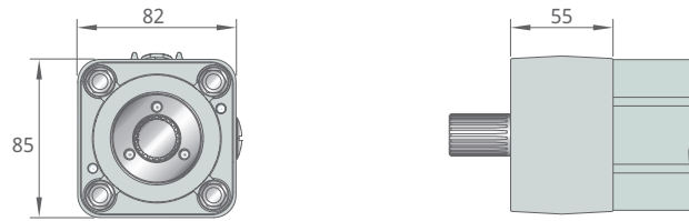
19 Dimensions of bearing housing without attachment
