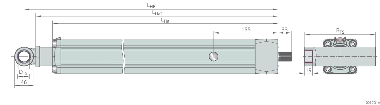
4 Dimensions with T-bar on push tube
