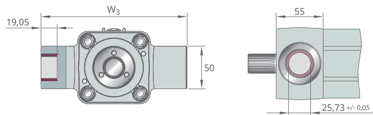
21 Dimensions of bearing housing with female trunnion mount
