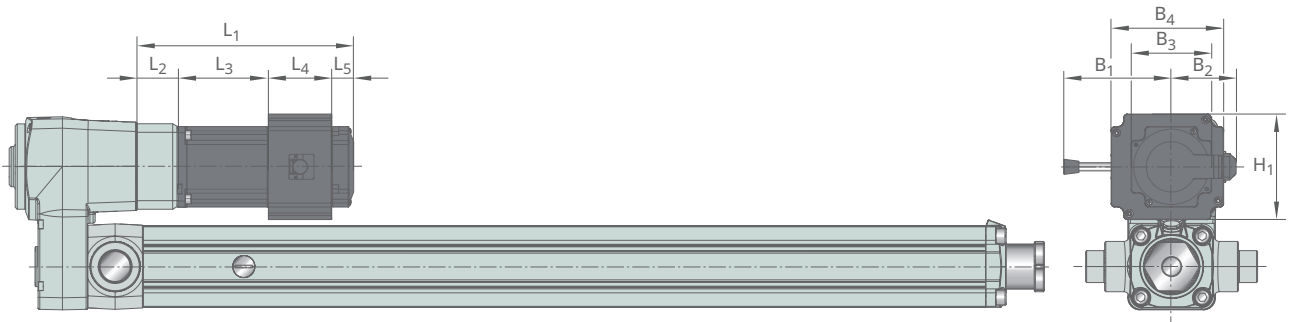
46 Dimensions for 750-W servo motor Fulling FL80SV75
