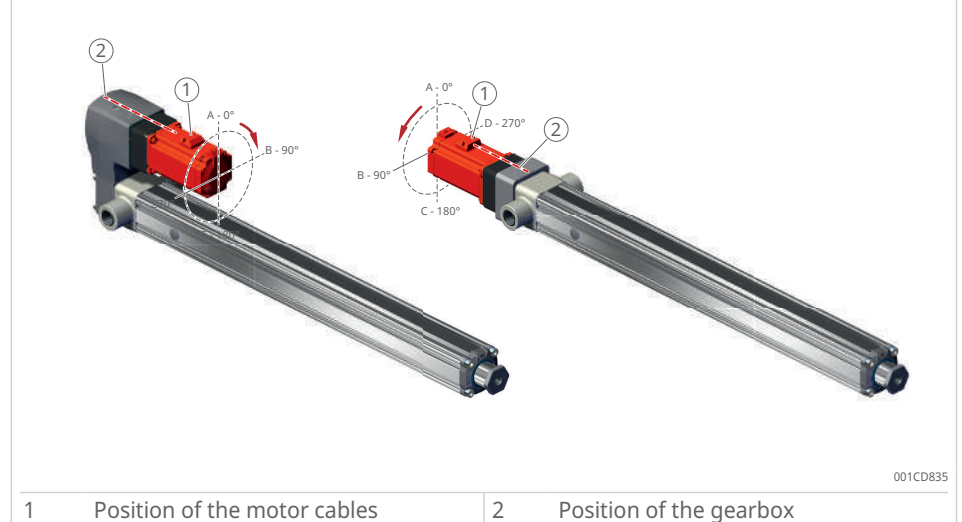
49 Motor orientation relative to gearbox
