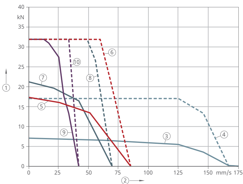
42 Speed-load diagram for 1 kW motor
