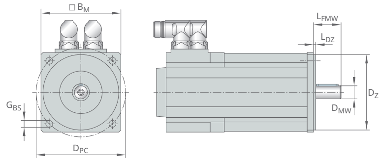
36 Motor adapter dimensions for inline gearbox and 3-stage spur gearbox
