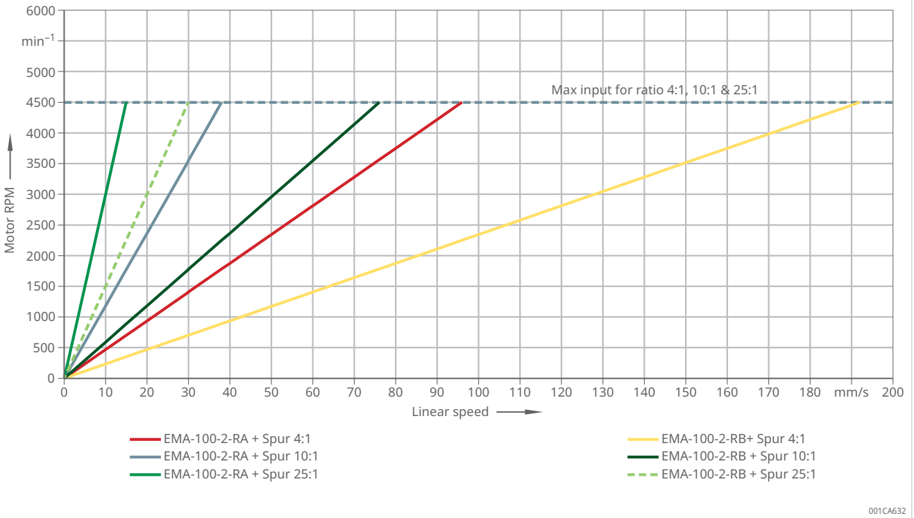
13 Required motor RPM to reach Linear speed (mm/s) EMA-100-2-R + Spur gearbox (4:1, 10:1 & 25:1)
