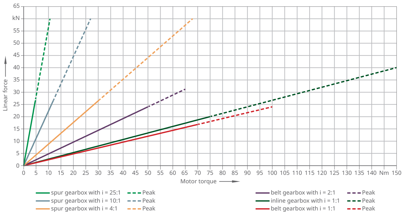
7 Motor torque and resulting linear force EMA-100-1-BC
