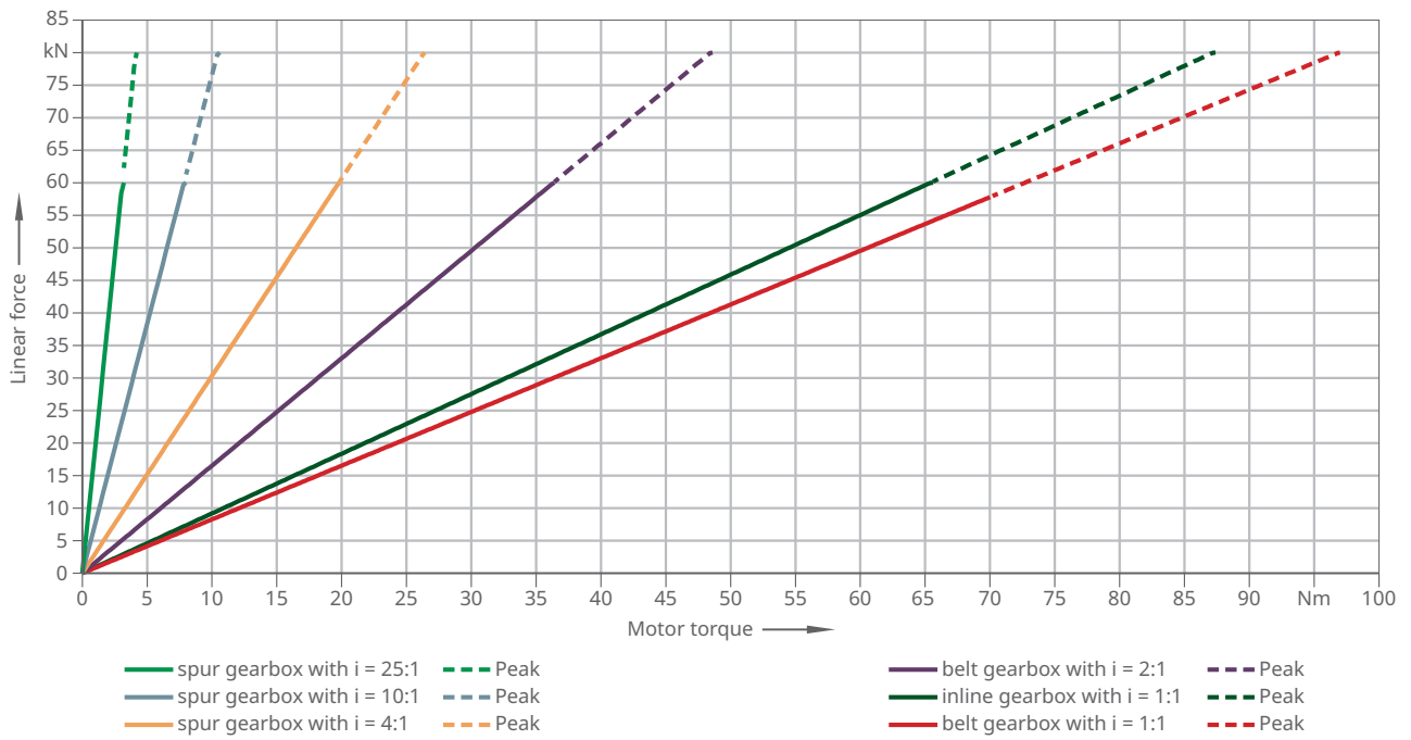
10 Motor torque and resulting linear force EMA-100-2-RA
