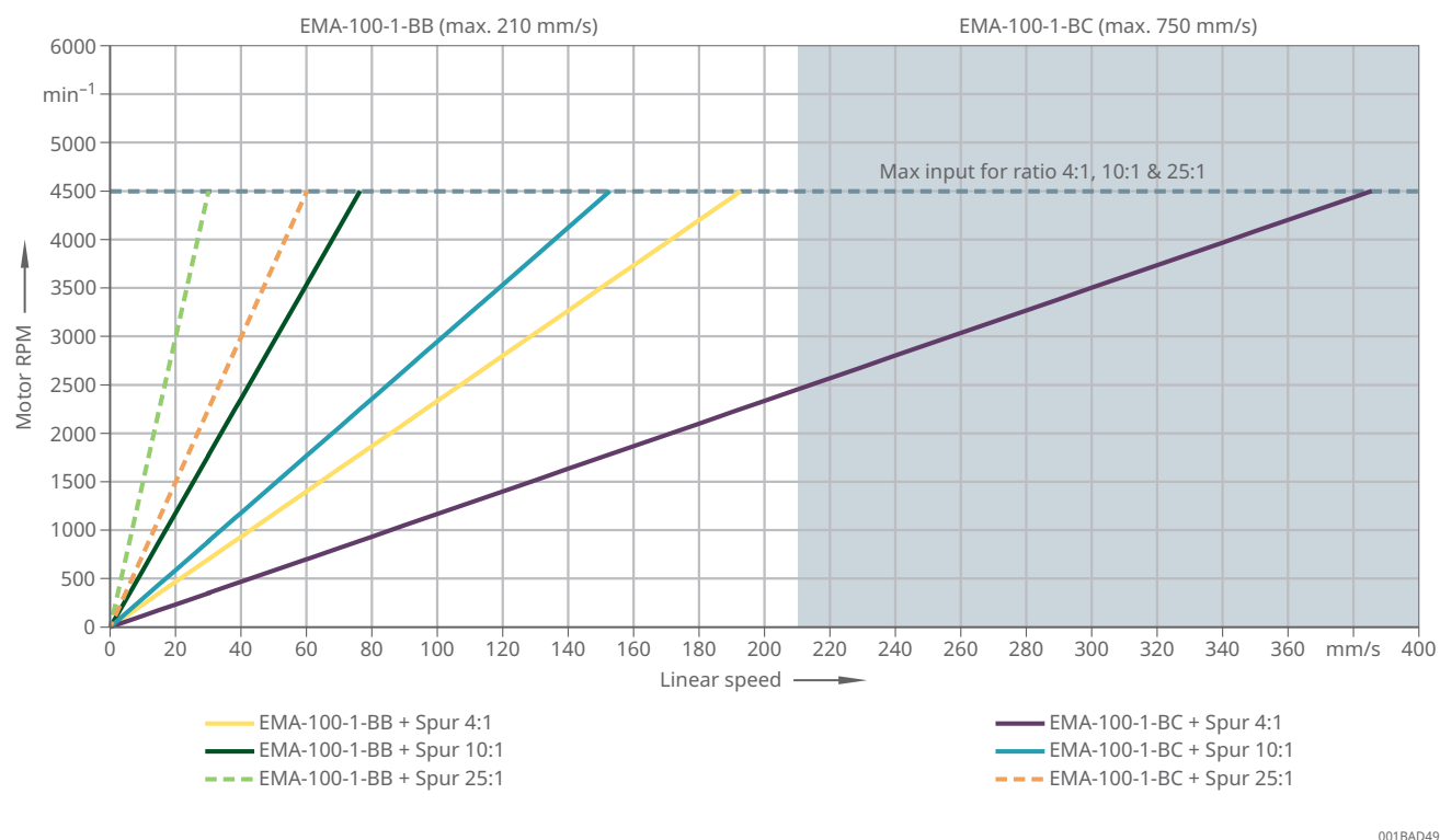
9 Required motor RPM to reach Linear speed (mm/s) EMA-100-1 + Spur gearbox (4:1, 10:1 & 25:1)
