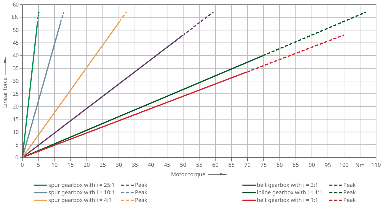
6 Motor torque and resulting linear force EMA-100-1-BB
