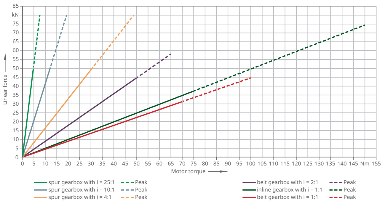
11 Motor torque and resulting linear force EMA-100-2-RB
